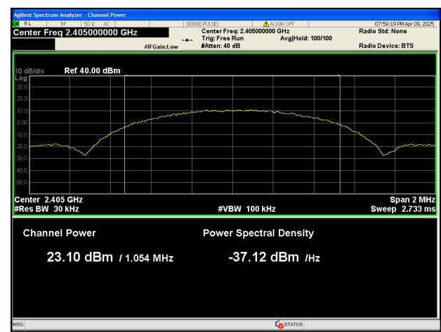
Mode: TX GFSK channel 0
