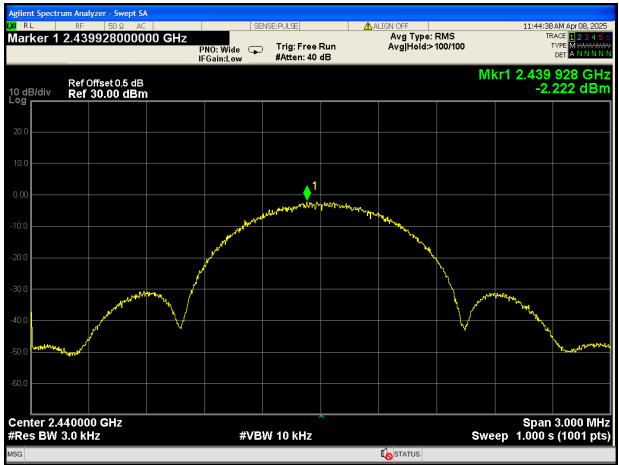
Mode: TX GFSK channel 11
