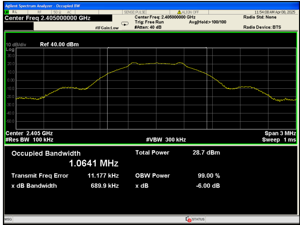
Mode: TX GFSK channel 0
