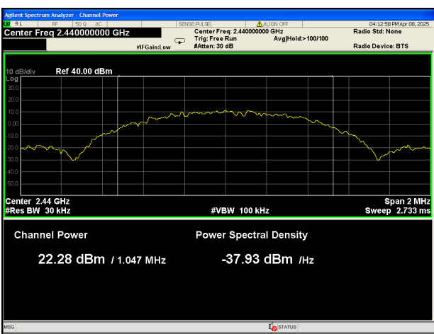
Mode: TX GFSK channel 11
