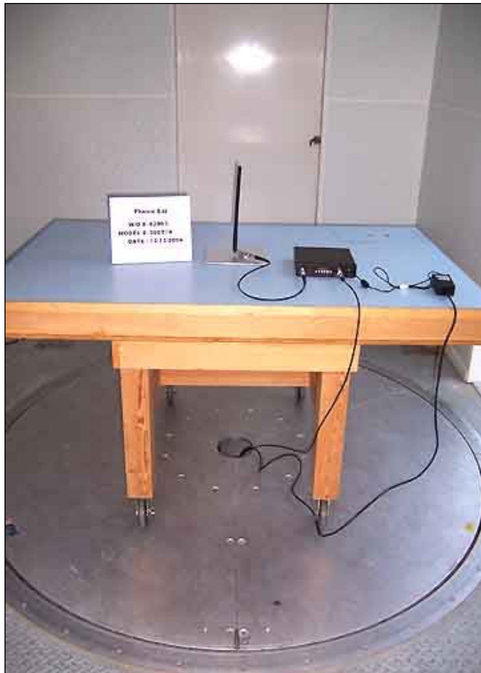
Radiated Emissions - Back View - Antenna B
