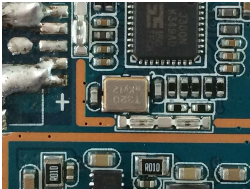
Oscillator 3 view
