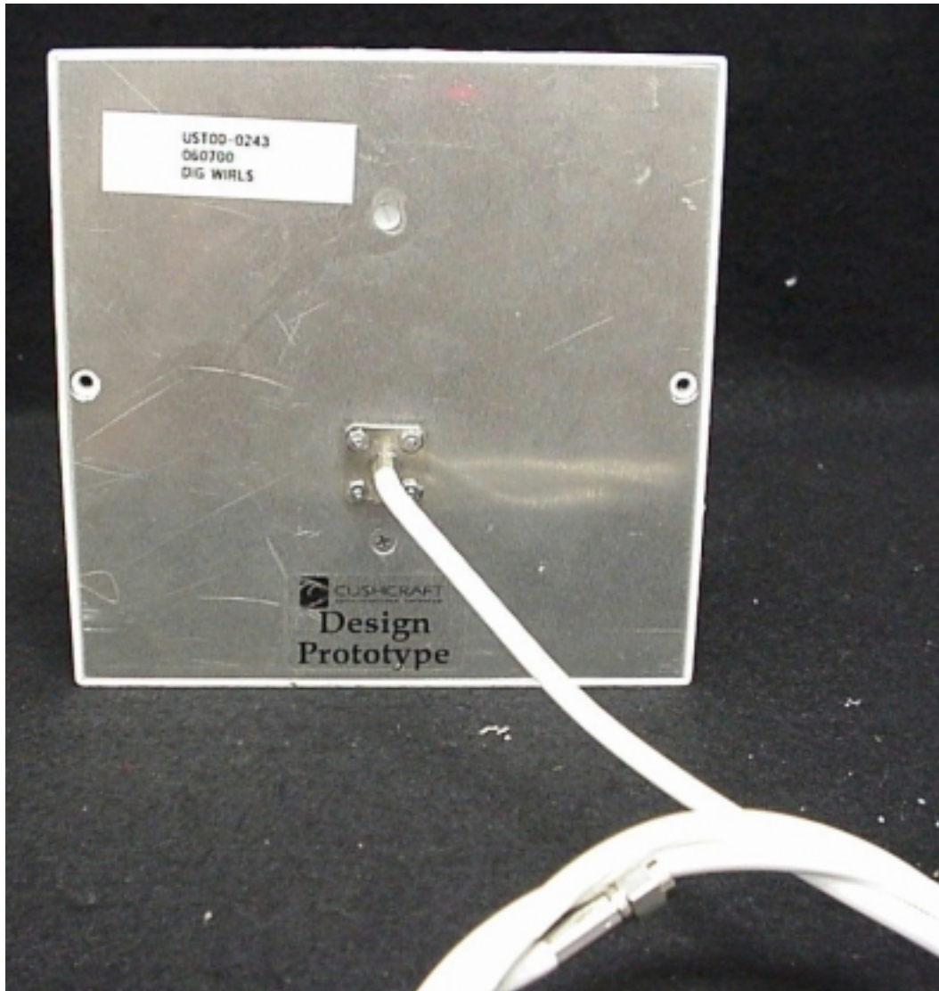
Photo 12. Patch Antenna, Bottom View
