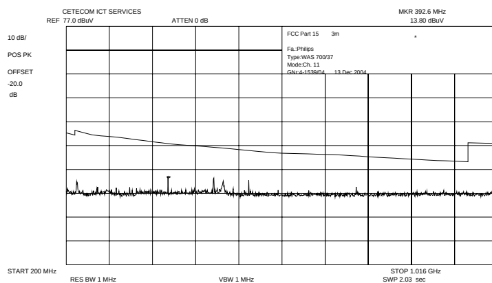
Plot 11: 200 MHz – 1000 MHz horizontal / vertical (highest channel)
