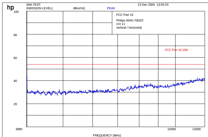
Plot 13: 4 – 12 GHz horizontal / vertical (highest channel)
