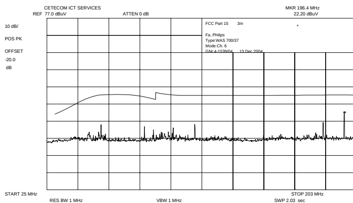
Plot 6: 30 - 200 MHz vertical / horizontal (middle channel)
