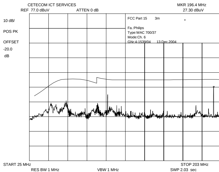
Plot 6: 30 - 200 MHz vertical / horizontal (middle channel)
