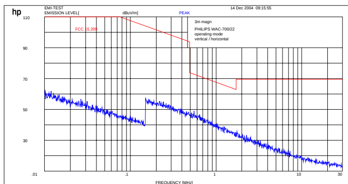
Plot 1: 9 kHz – 30 MHz radiated emissions
