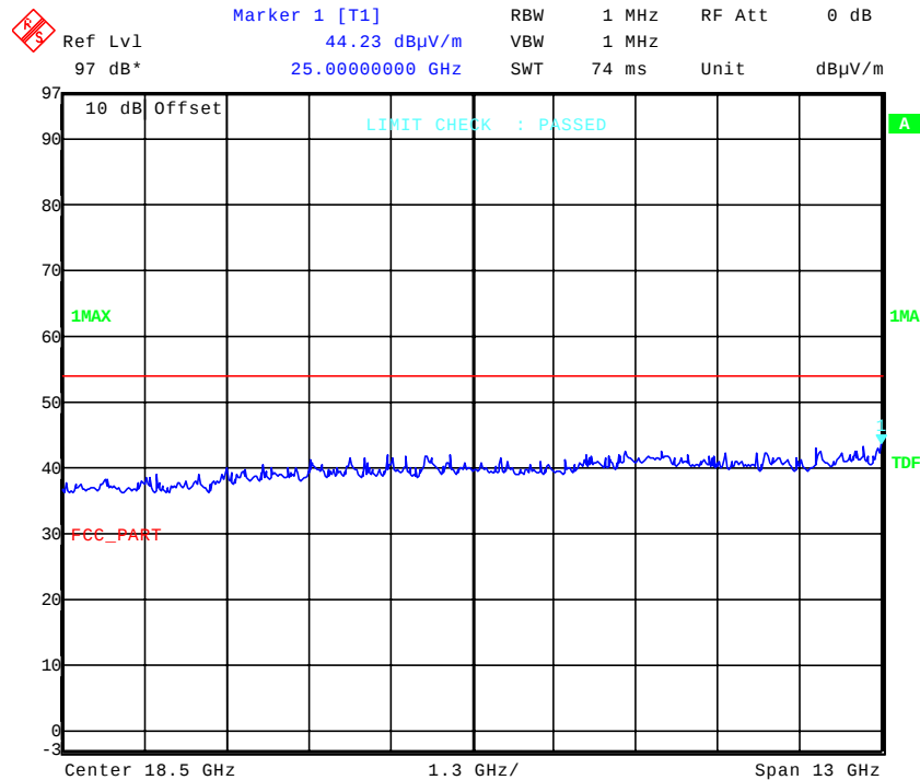
Plot 5: 12 – 25 GHz horizontal / vertical (lowest channel), valid for all three channels
