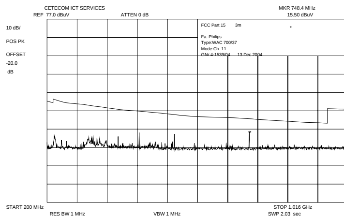
Plot 11: 200 MHz – 1000 MHz horizontal / vertical (highest channel)
