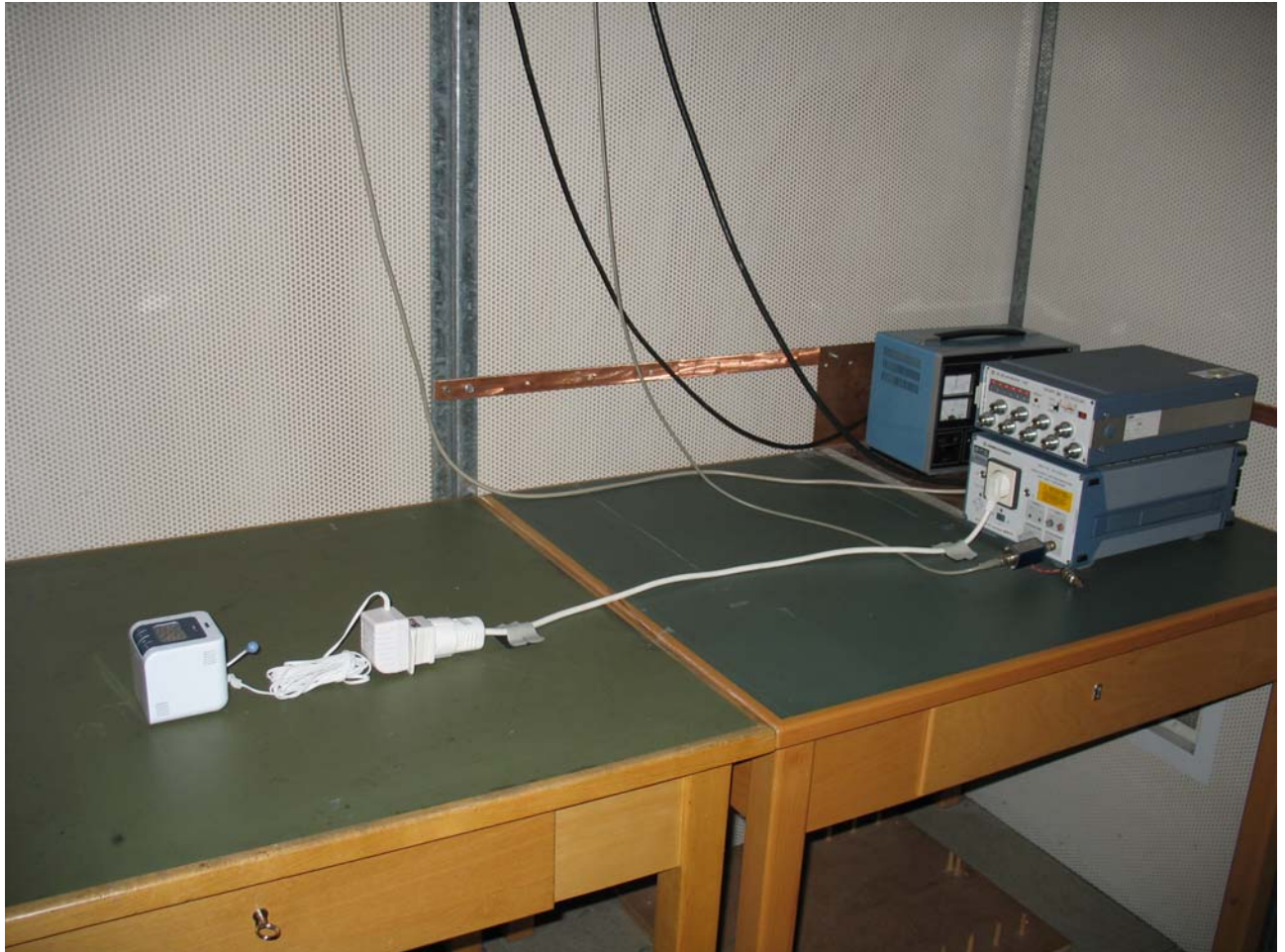
Photo 1: Power Line Conducted Emission Test
