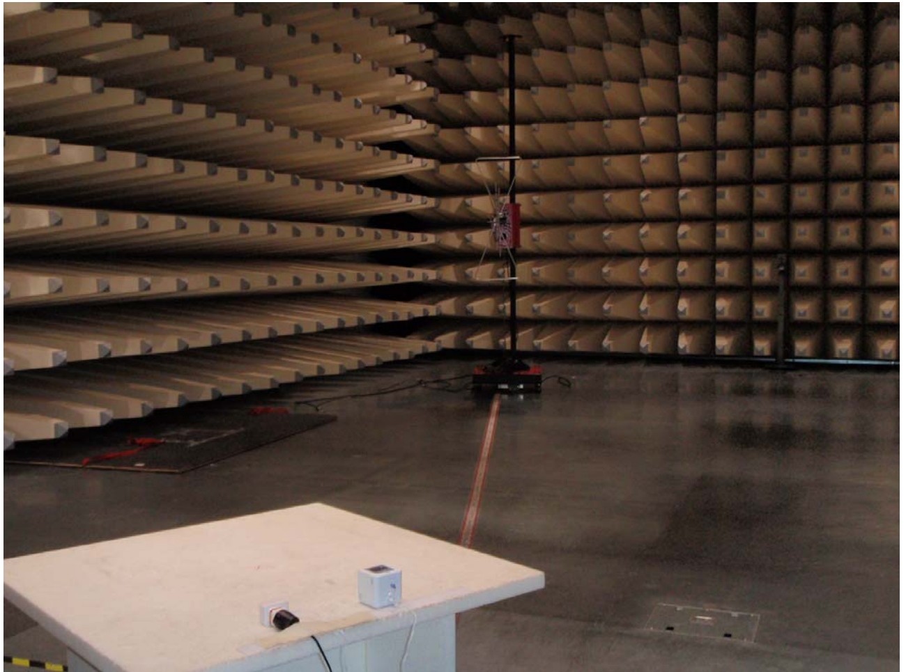
Photo 2: Radiated Emission
