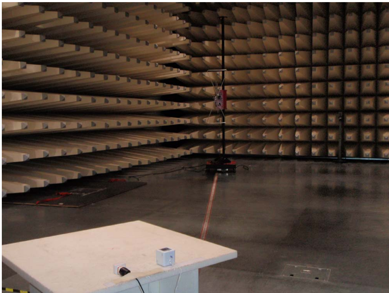
Photo 2: Radiated Emission
