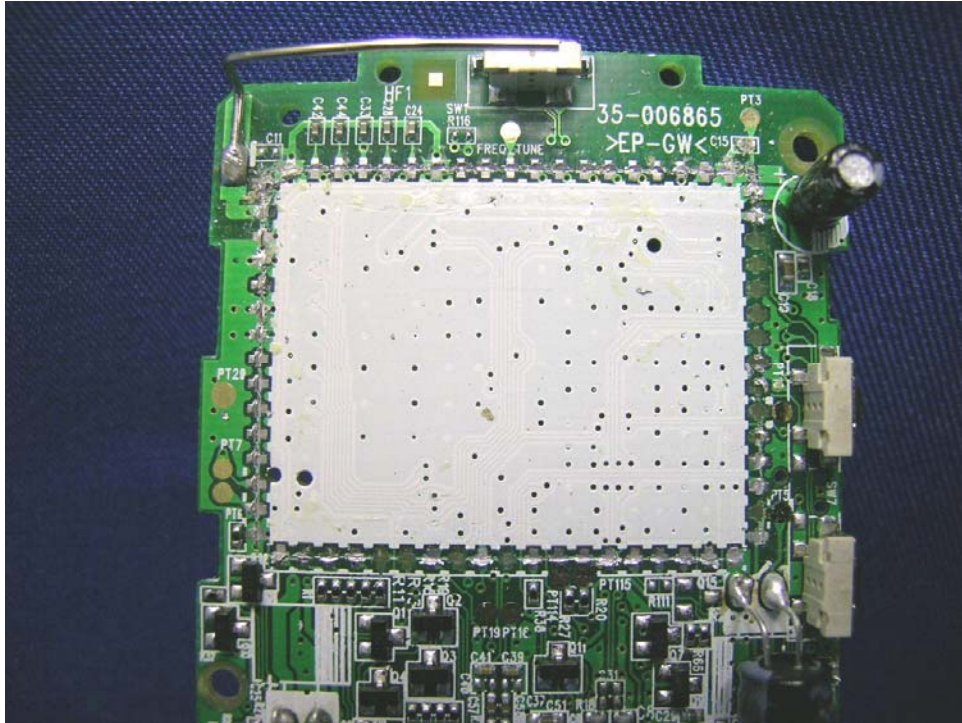
Main PCB comp side (View 3)
