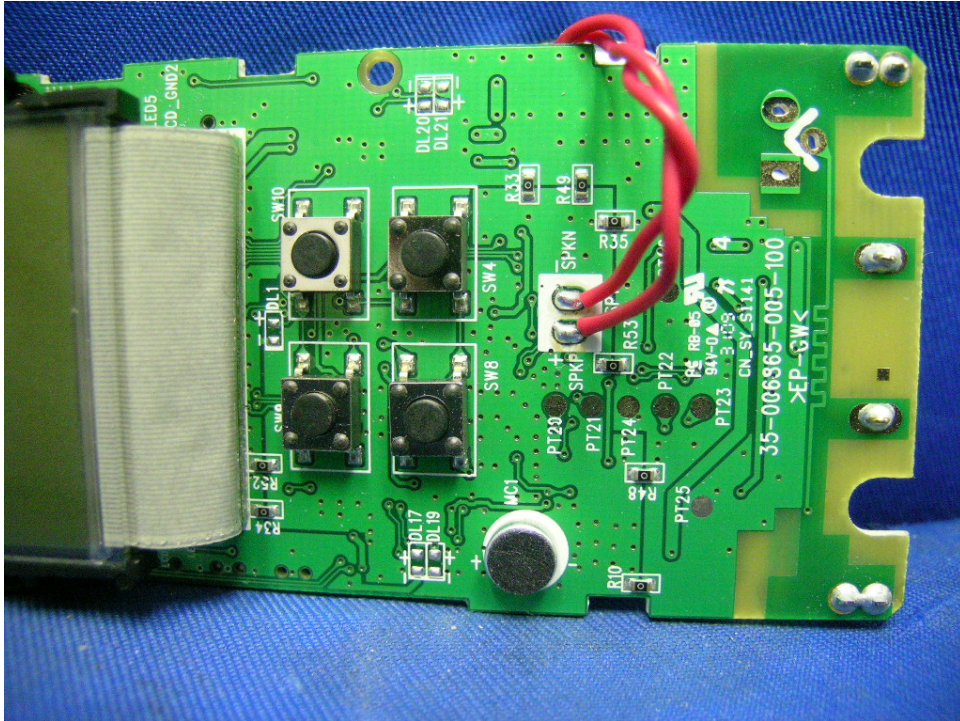
Main PCB solder side (View 2)
