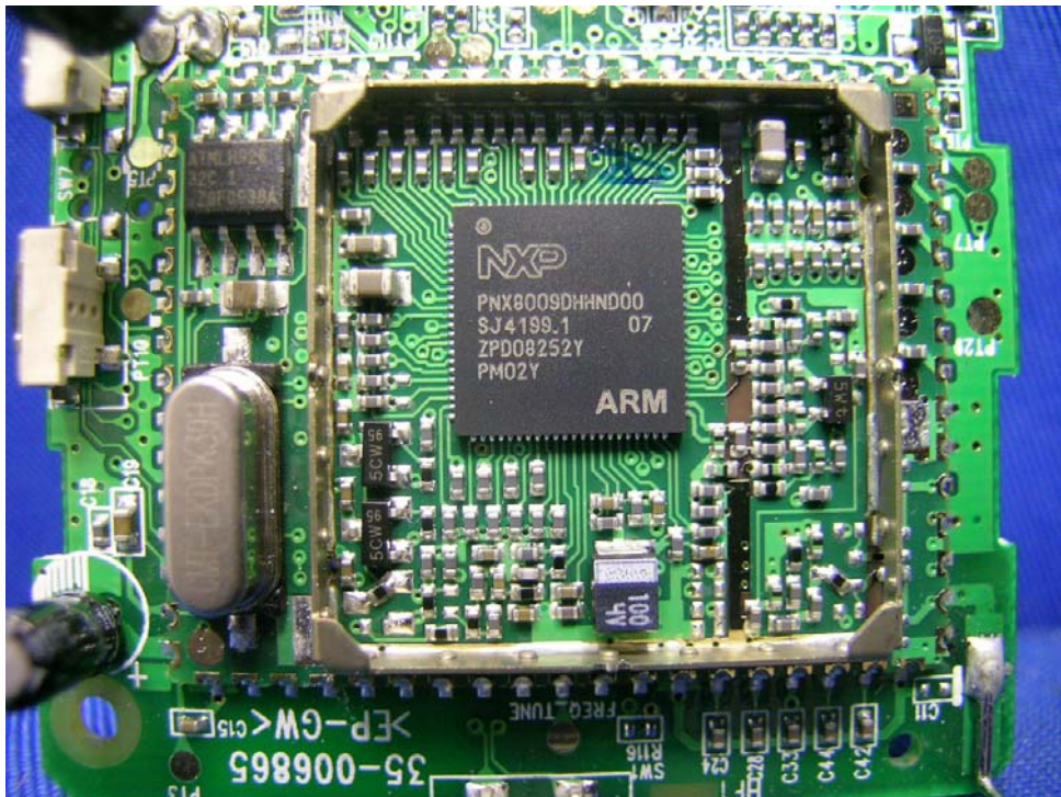
DECT RF Module comp side
