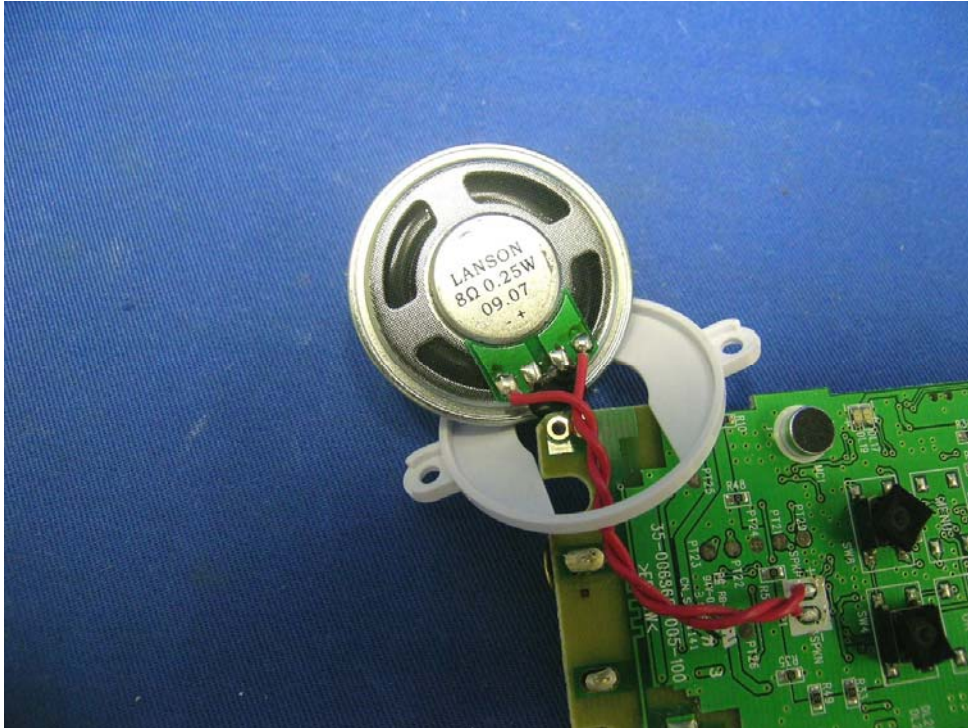
Speaker PCB
