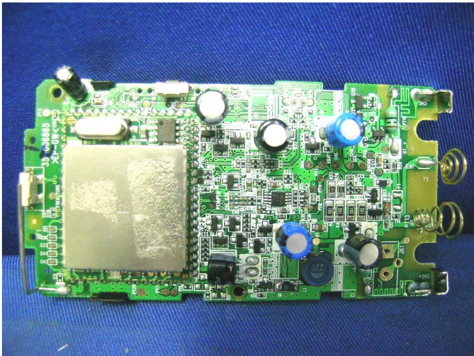
Main PCB comp side (view 2)
