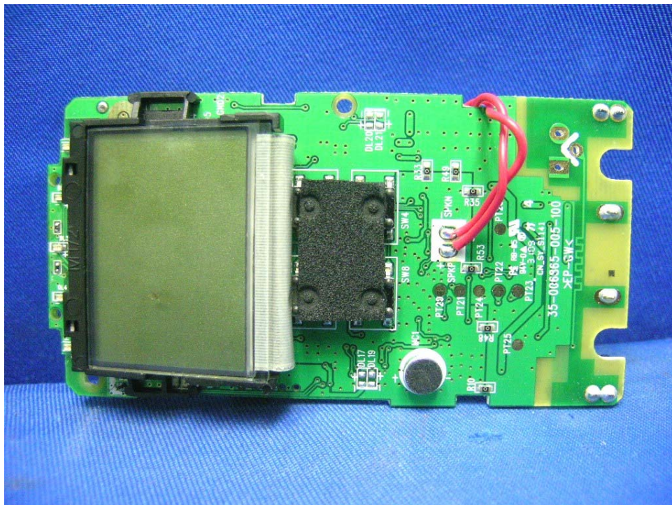
Main PCB solder side (View 1)
