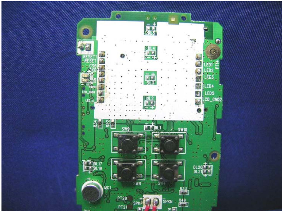
Main PCB solder side (View 3)
