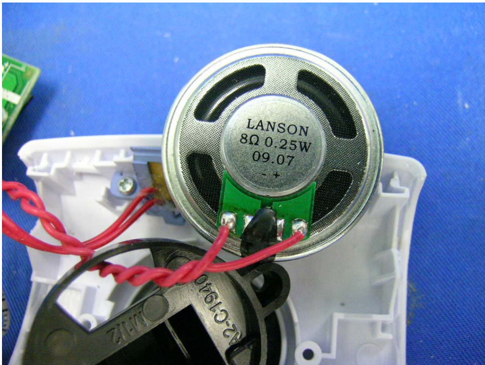
Baby Unit Speaker PCB
