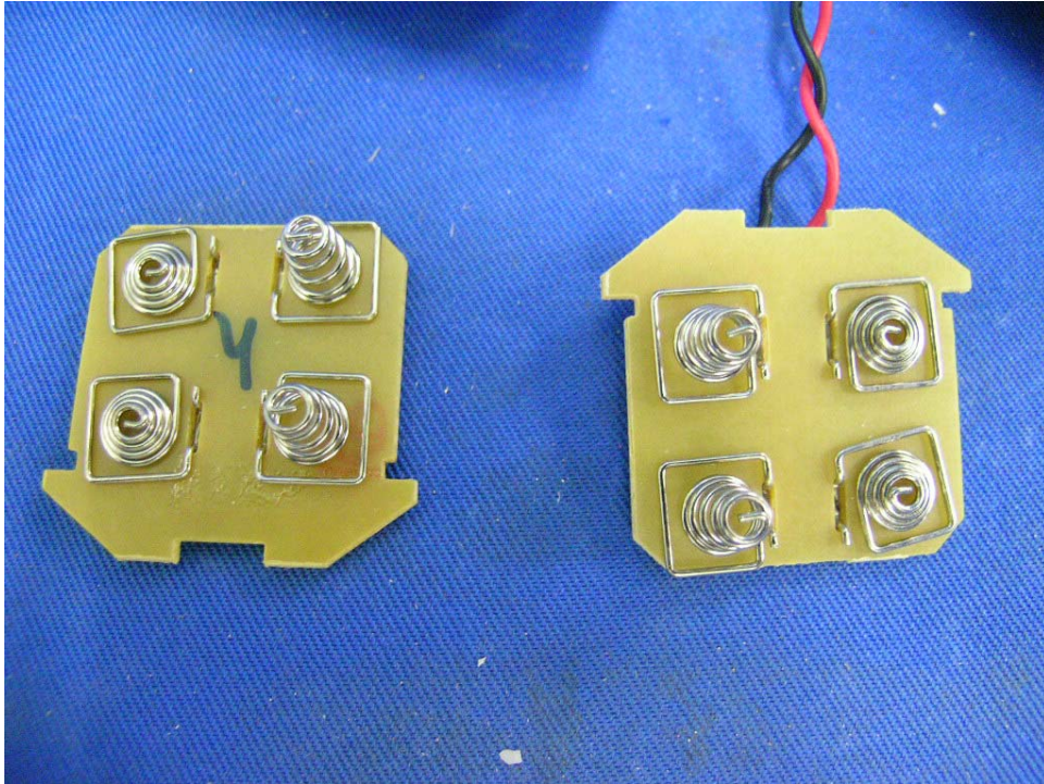
Baby Unit Battery Contact PCB front side
