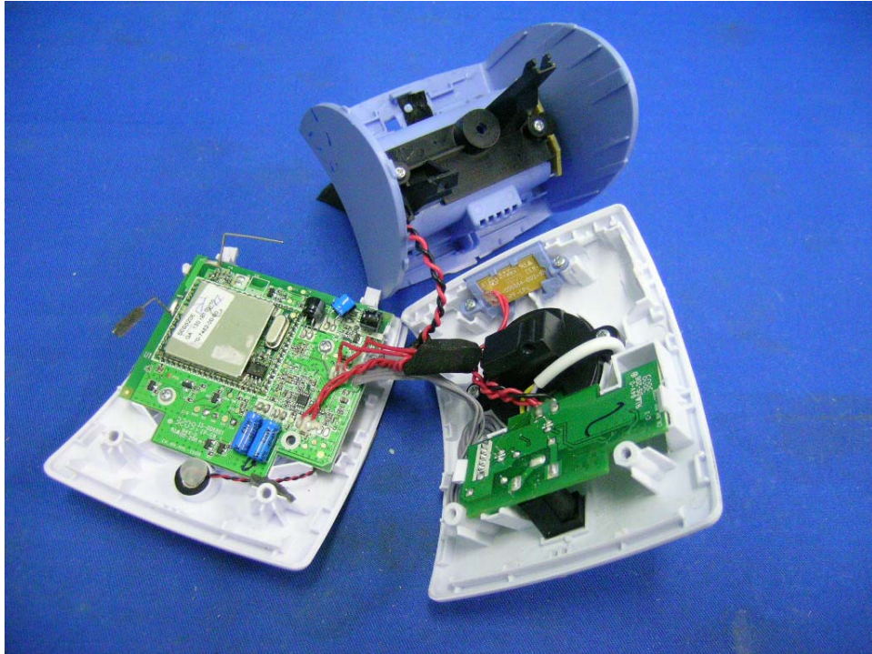
Baby Unit assembly (View 1)
