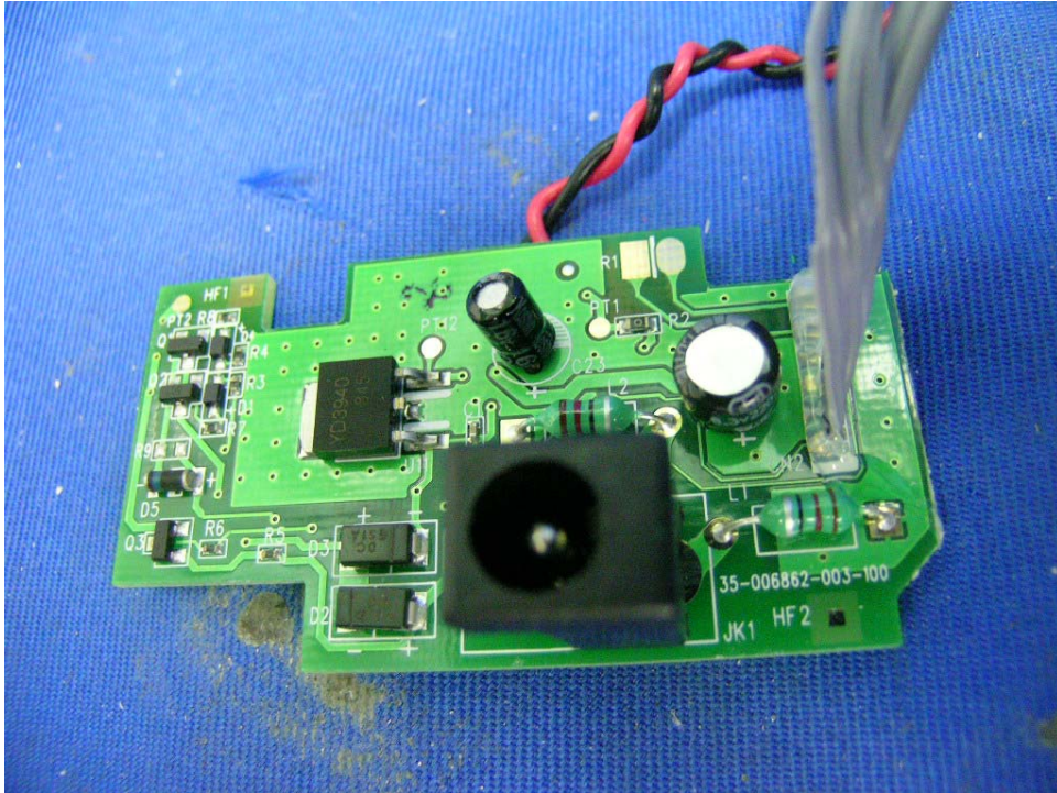
Baby Unit Power Supply PCB front side
