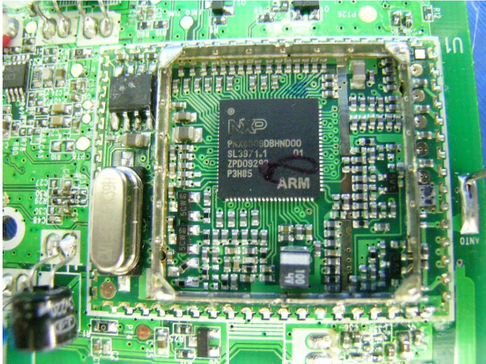
Baby Unit DECT RF Module comp side
