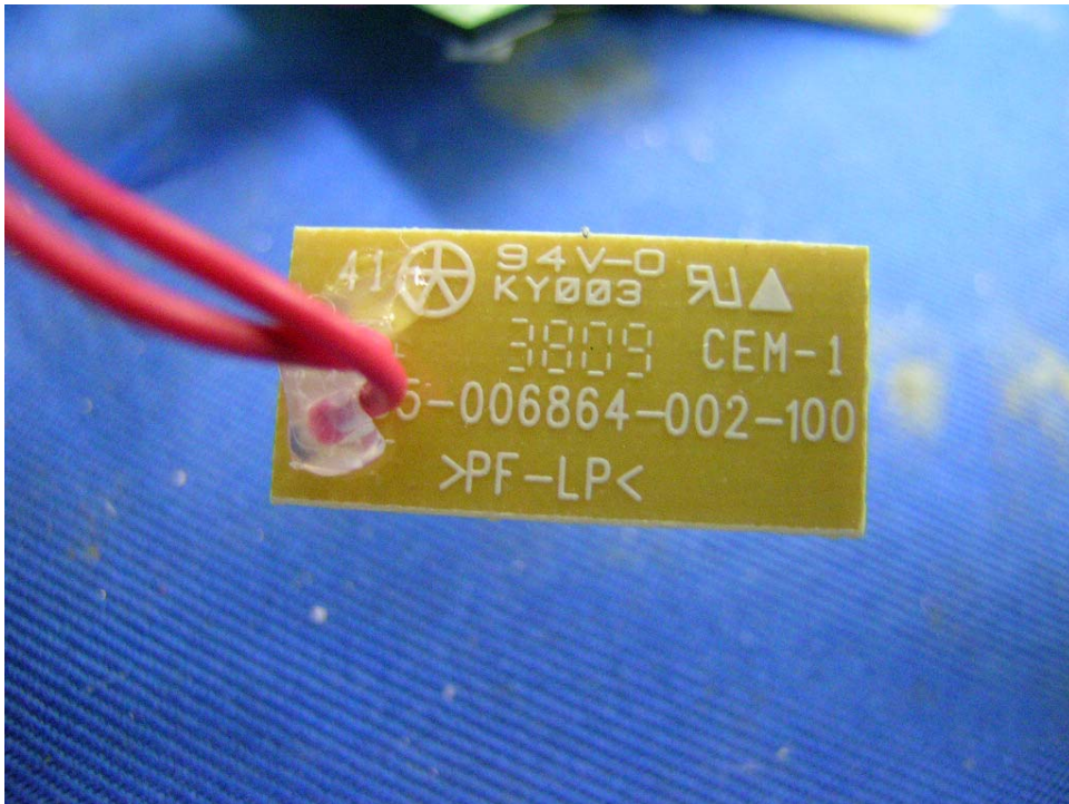
Baby Unit Power Button PCB rear side
