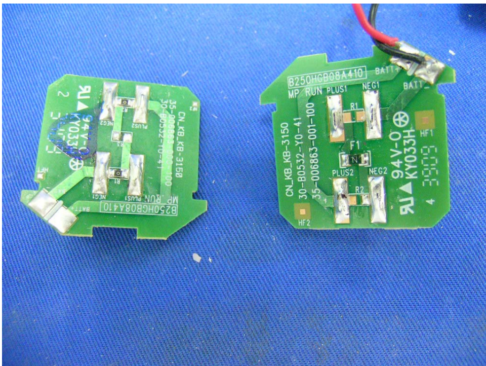
Baby Unit Battery Contact PCB rear side
