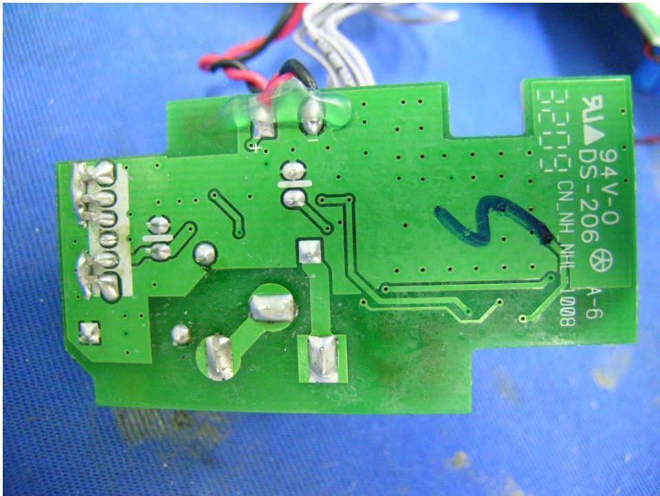
Baby Unit Power Supply PCB rear side
