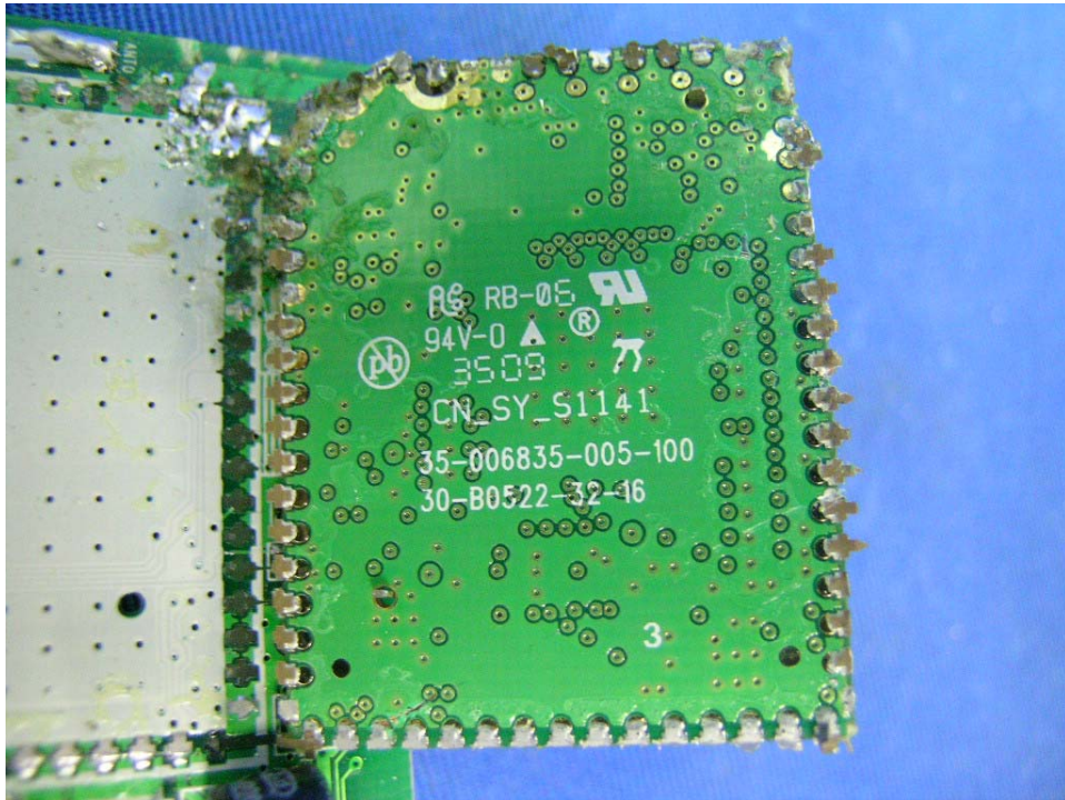
Baby Unit DECT RF Module solder side
