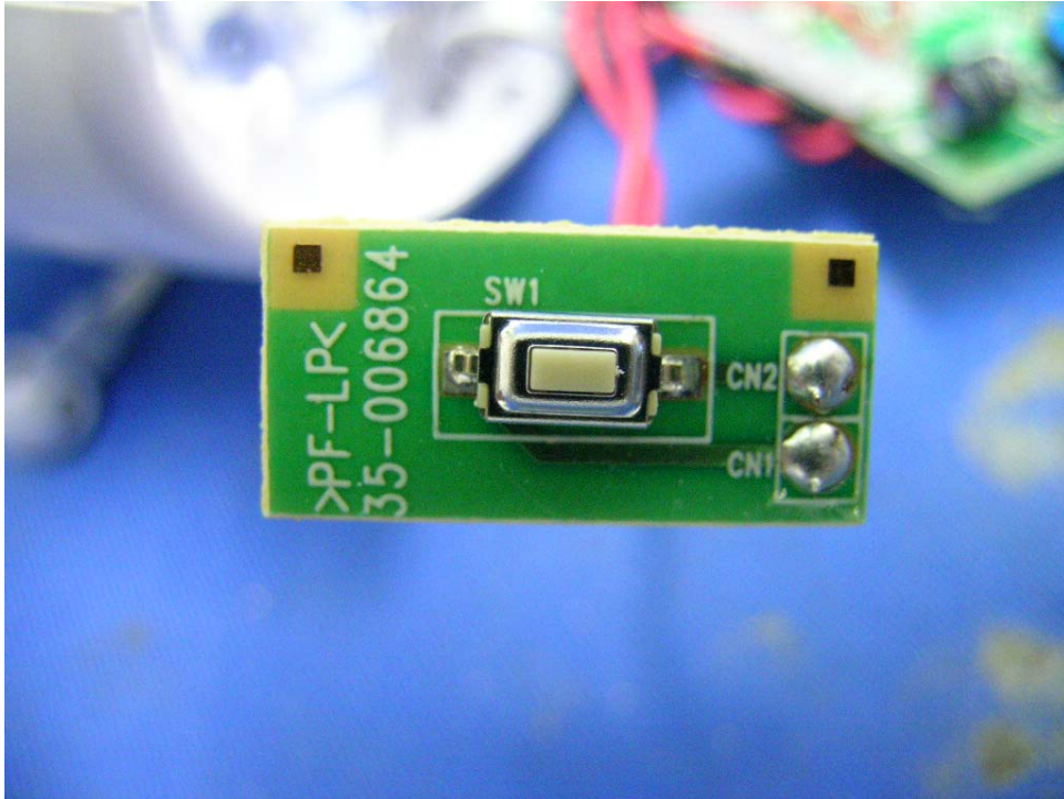
Baby Unit Power Button PCB front side
