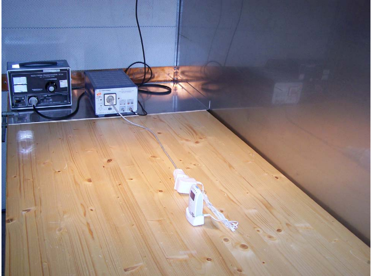
Photo 1: Power Line Conducted Emission Test
