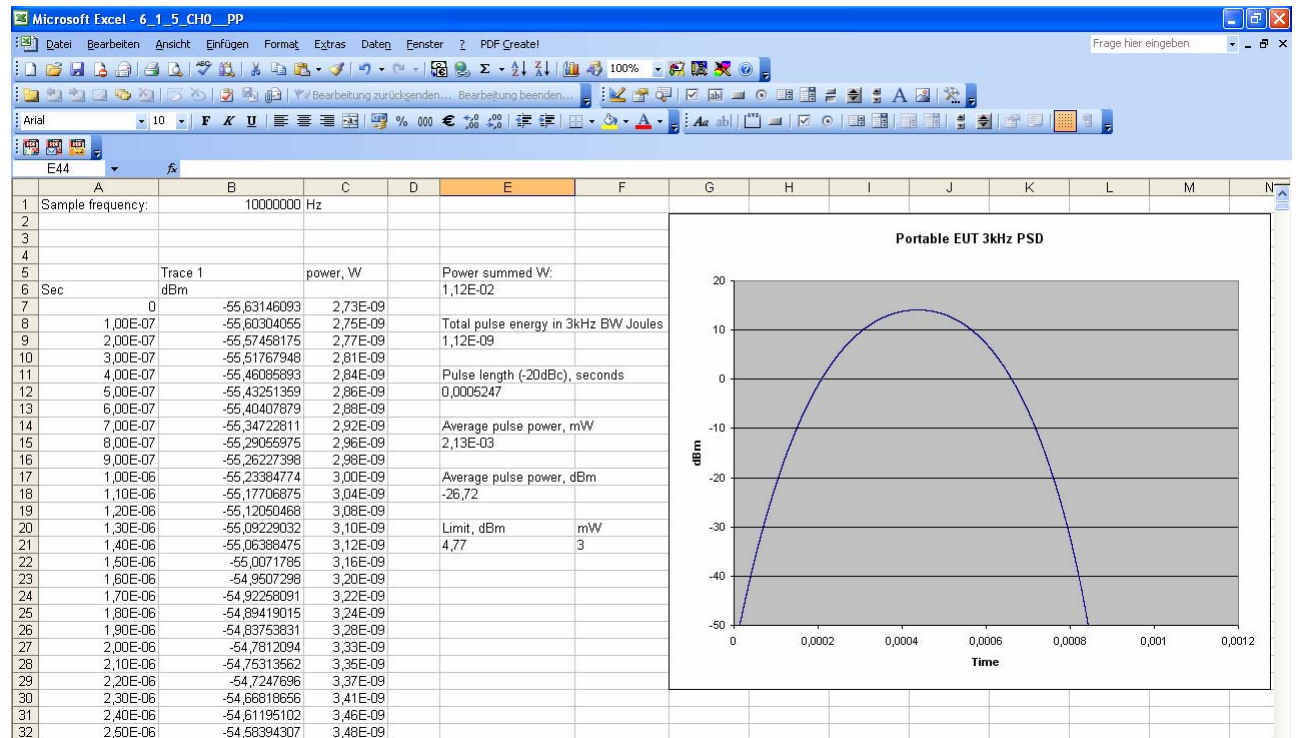
Screenshot of Excel file showing PSD calculations for portable EUT, Upper Channel
