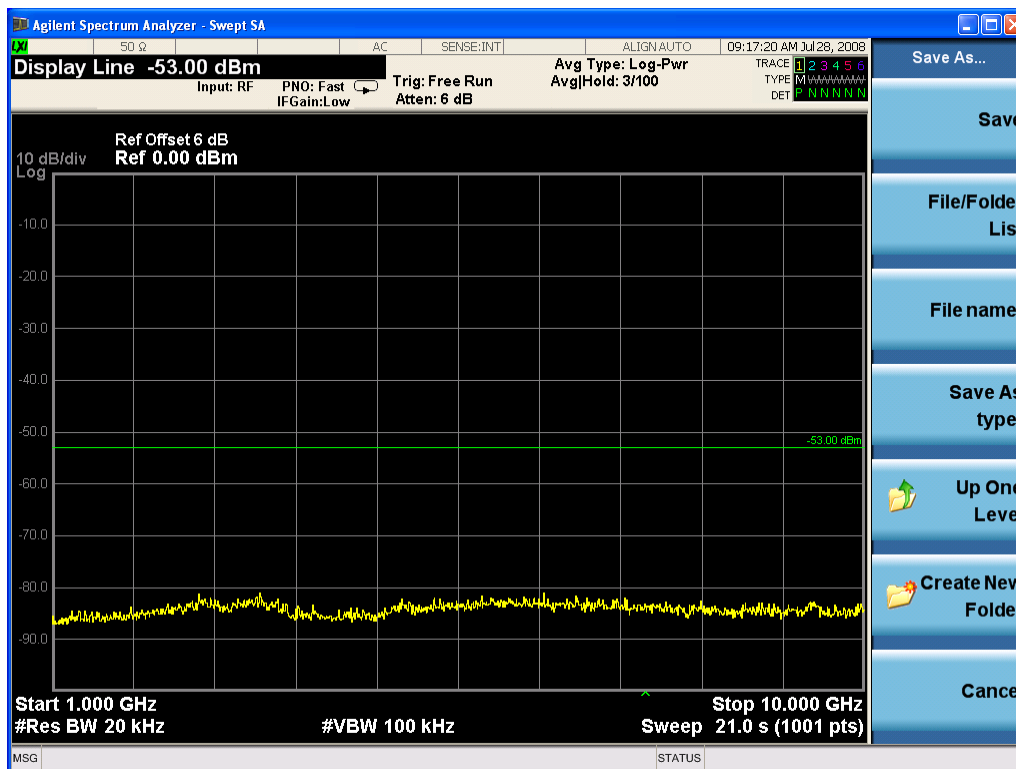
Receiver Spurious Emissions, Conducted, 1 GHz – 10 GHz
