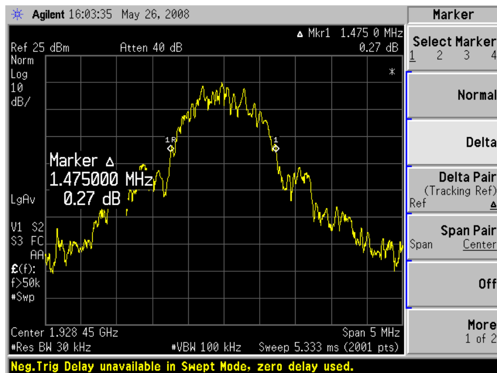
Emission Bandwidth B, Upper Channel
