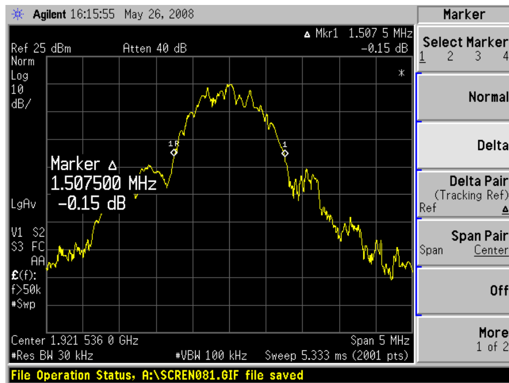
Emission Bandwidth B, Lower Channel
