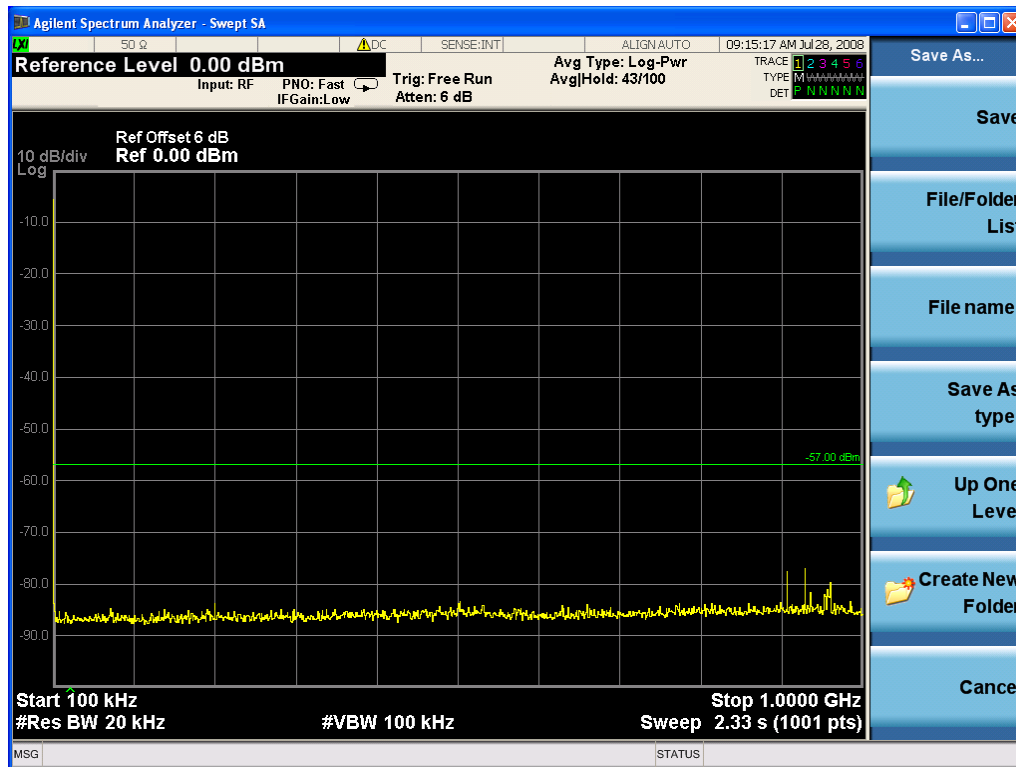
Receiver Spurious Emissions, Conducted, 100 kHz – 1 GHz
