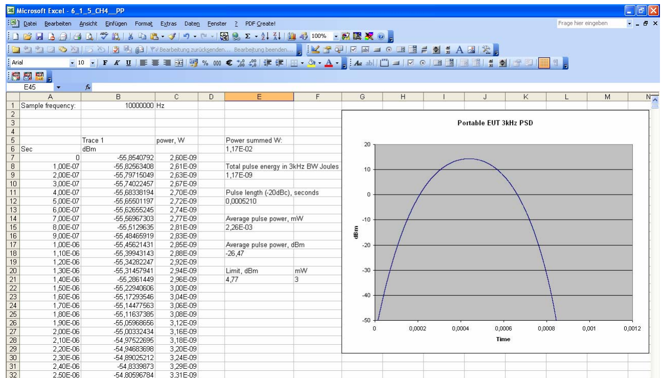
Screenshot of Excel file showing PSD calculations for portable EUT, Lower Channel
