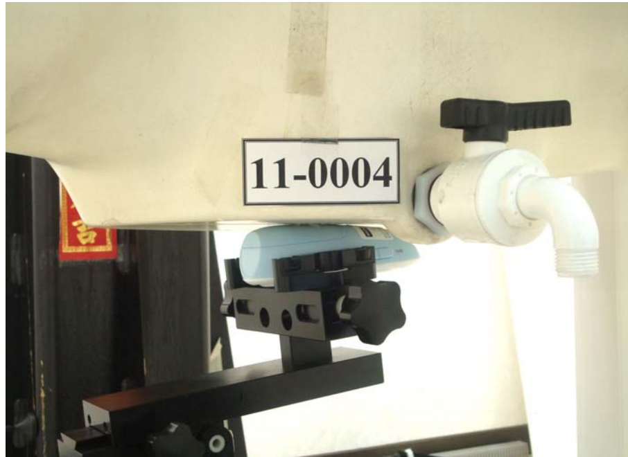
Figure 2. Body SAR Test Setup (Flat Section)
