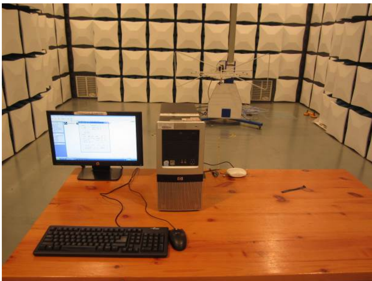
Figure 3 Radiated emission test setup (below 1 GHz)
