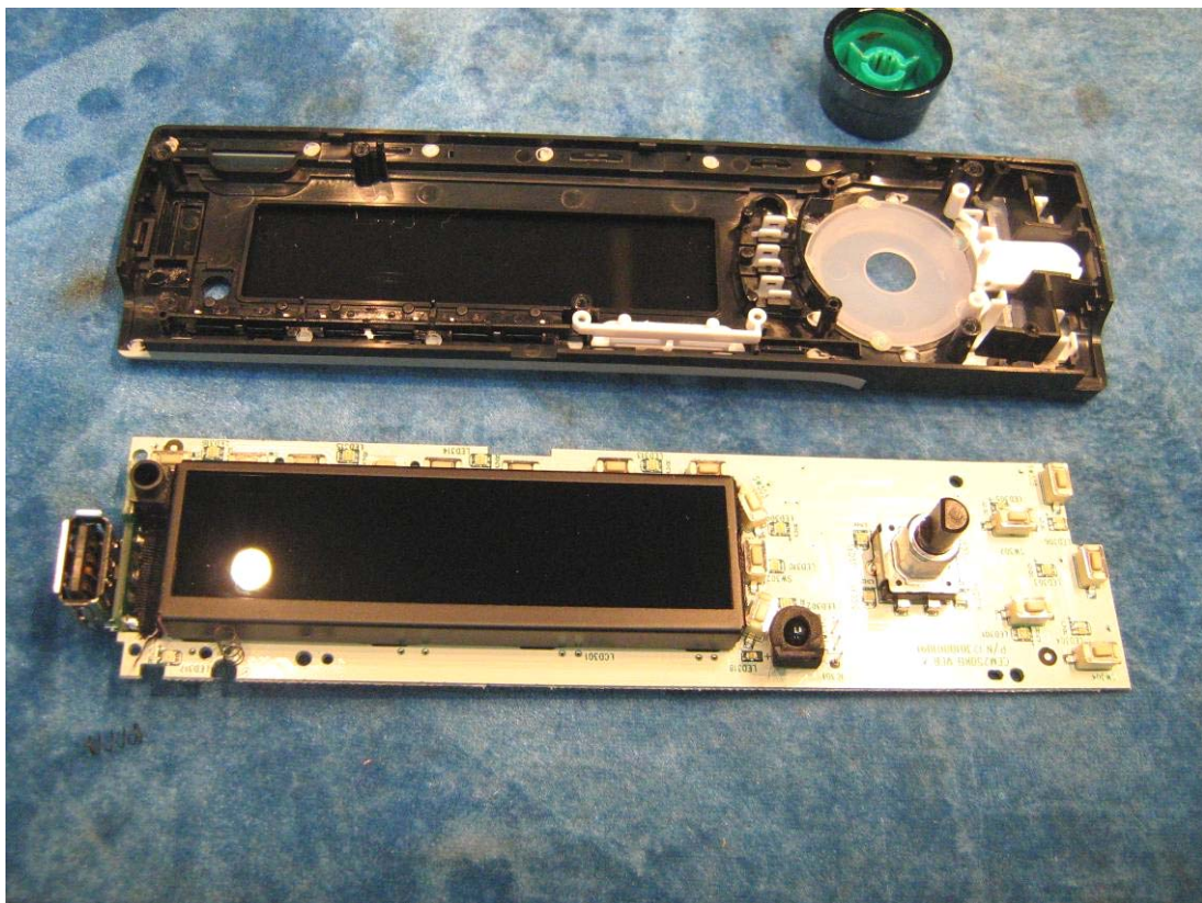
Picture 2 (internal view of panel)
