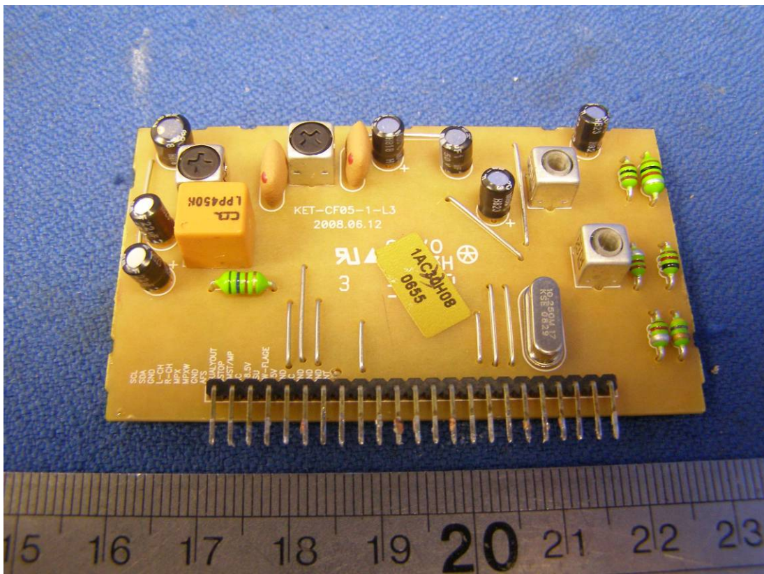
Picture 22 (front side of tuner board)
