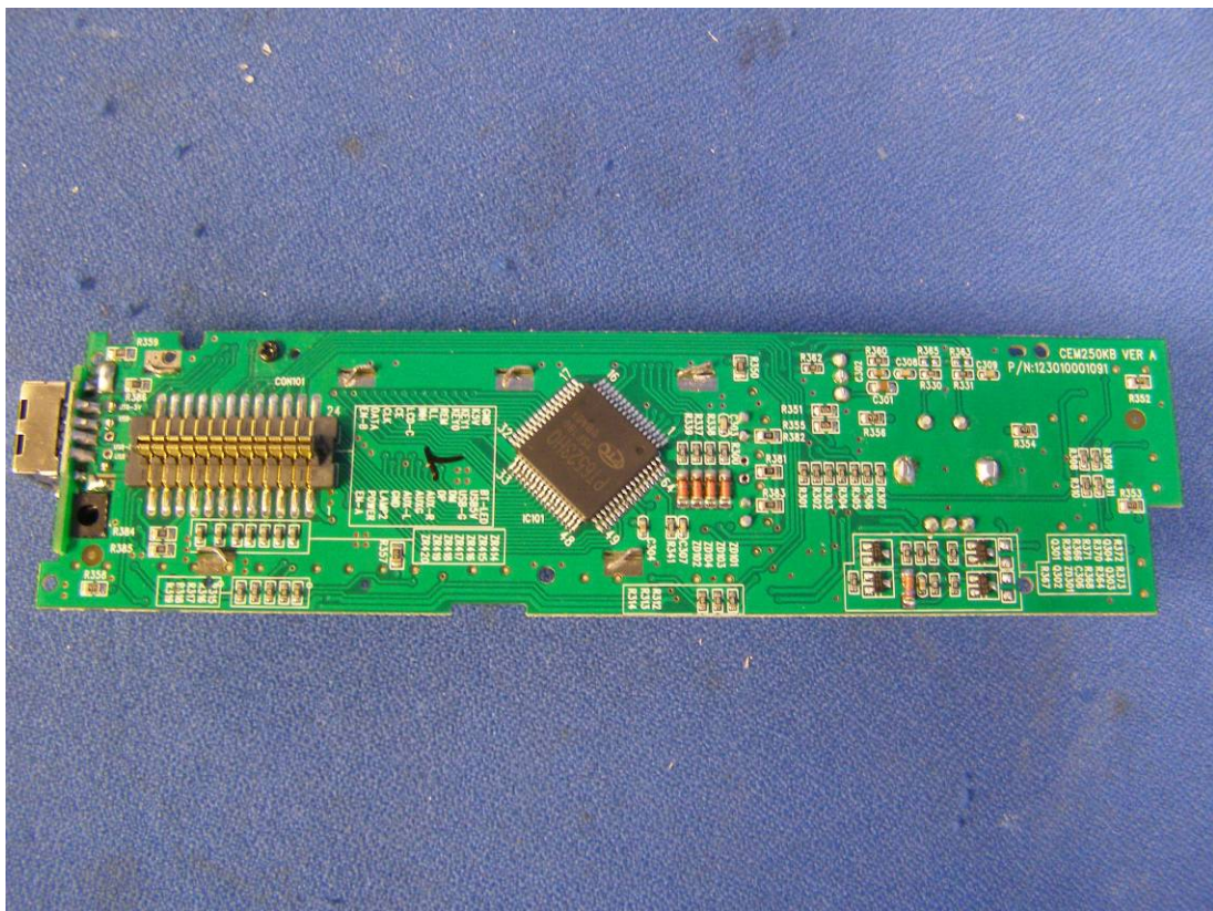
Picture 4 (back side of panel board)
