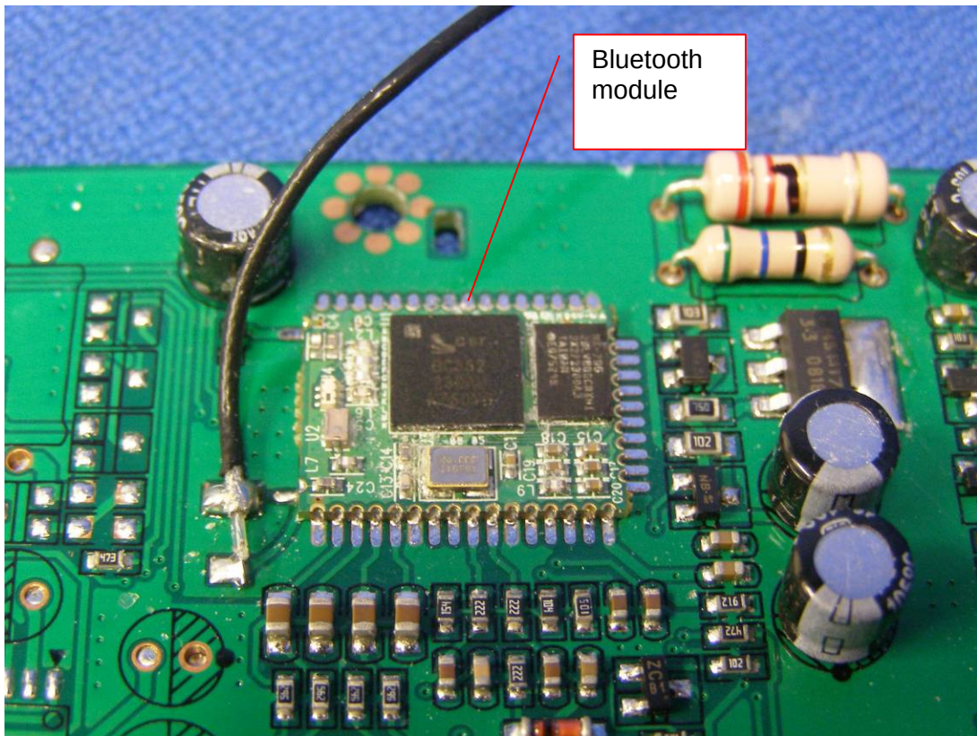
Picture 19 (Bluetooth module)
