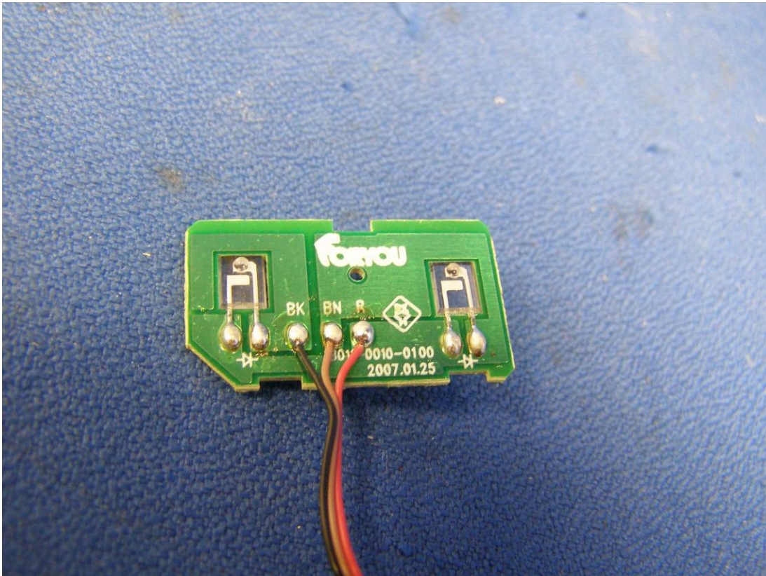
Picture 9 (front side of sensor board of CD deck)
