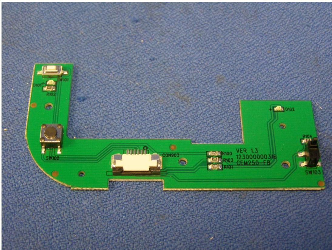
Picture 13 (front side of reset/eject board)
