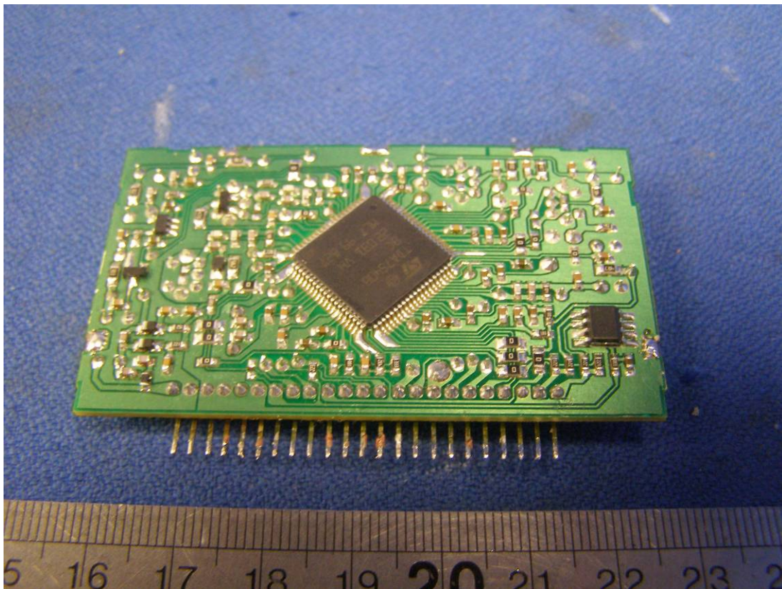
Picture 23 (back side of tuner board)
