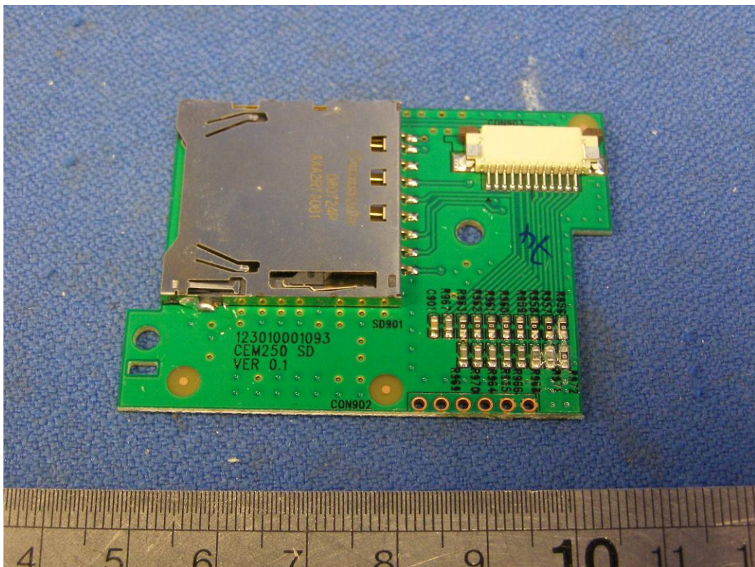
Picture 16 (front side of SD card board)
