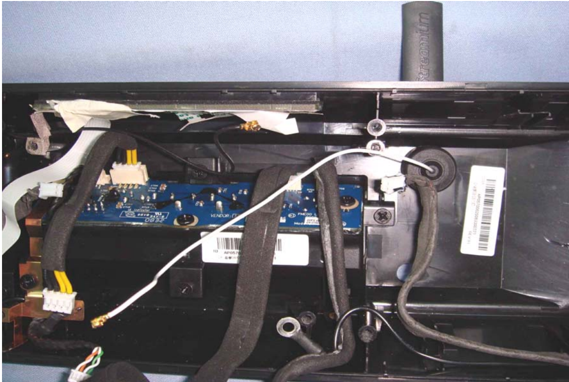
Dipole Antenna Location
