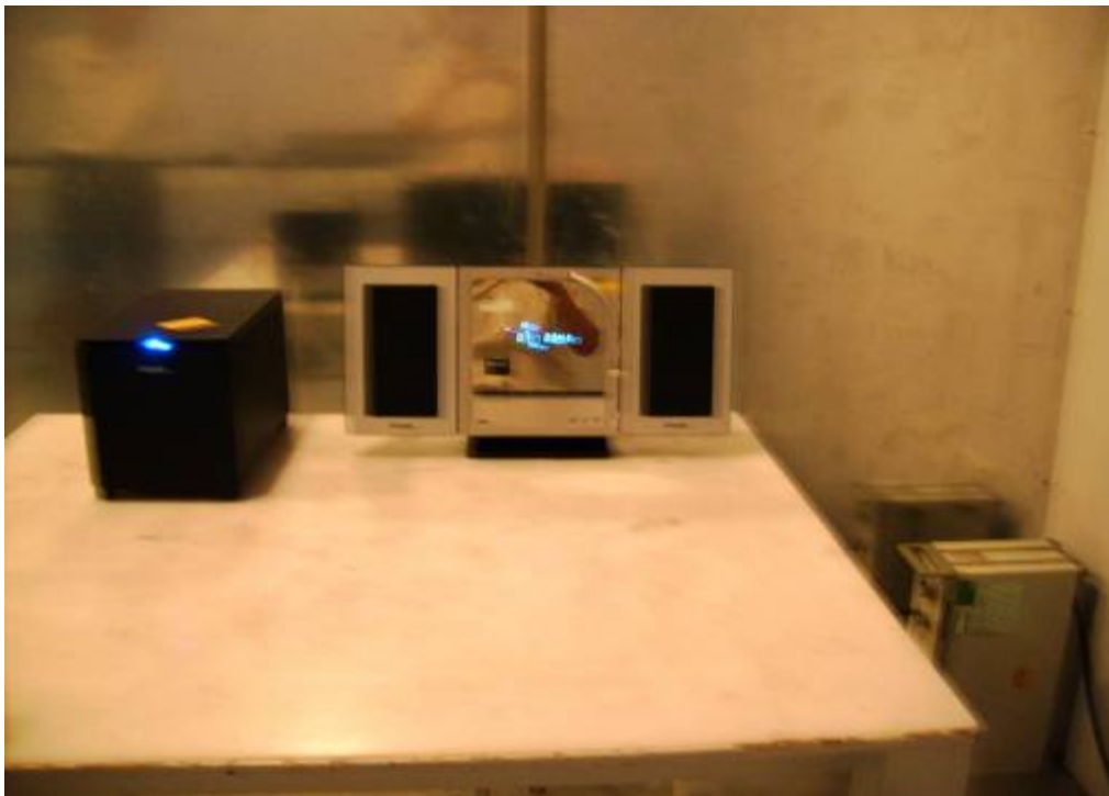
Conducted Emission Test Setup
