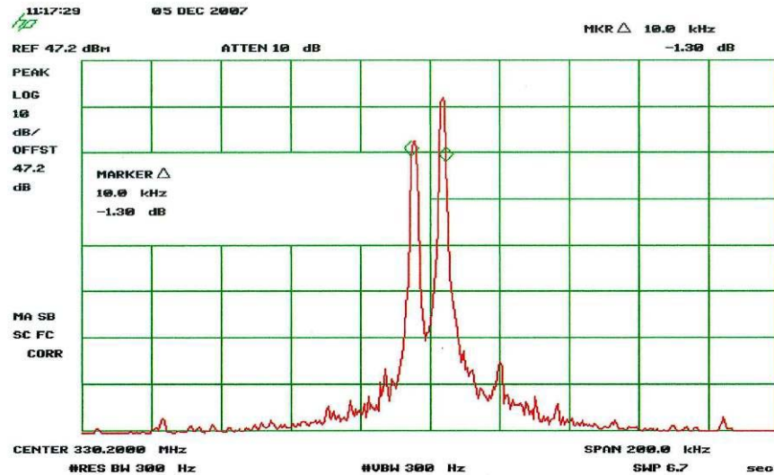
Figure 2: Occupied Bandwidth CLR @ 330.2MHz
