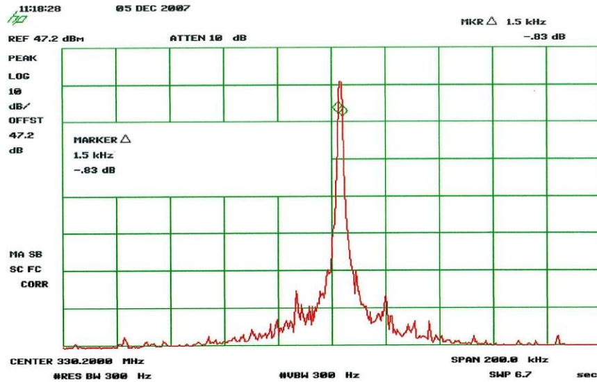
Figure 3: Occupied Bandwidth CRS @ 330.2MHz
