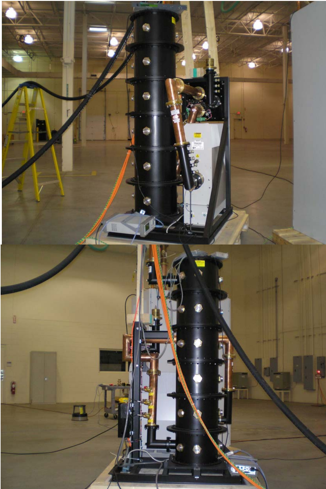
Photos of 12-Section Band-Pass Filter
