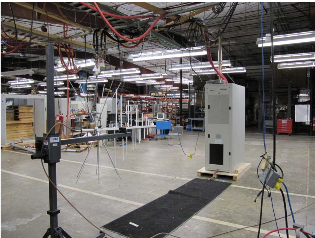
Biconicalog Antenna, Rear
