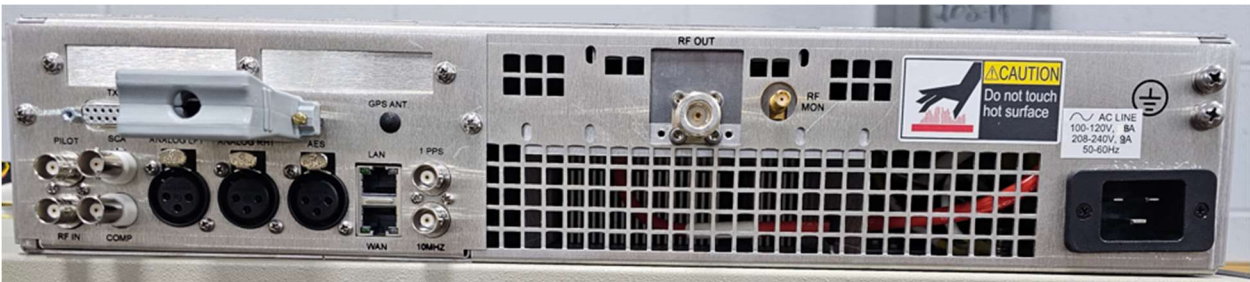
GX300 Rear:
