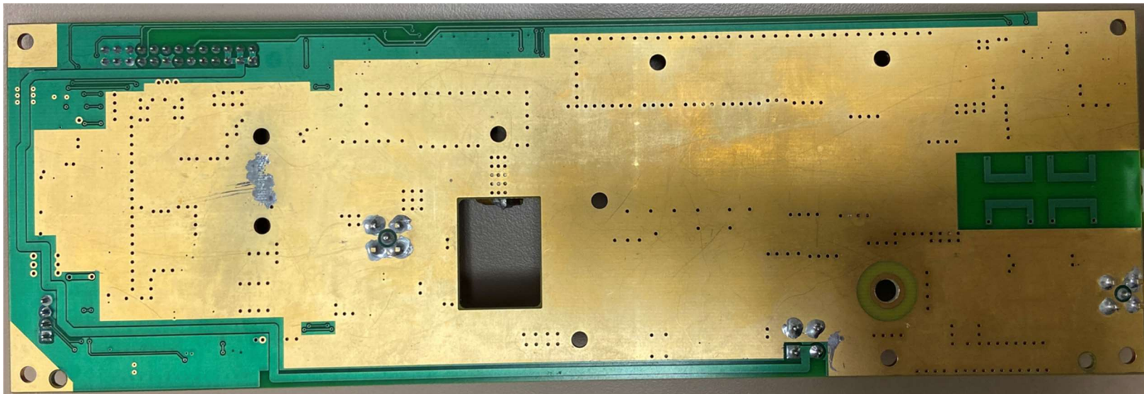
Bottom of 9010252511 PWA, PA GX150
