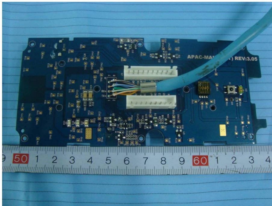
EUT – APAC-Main Board REV3.05 Top View
