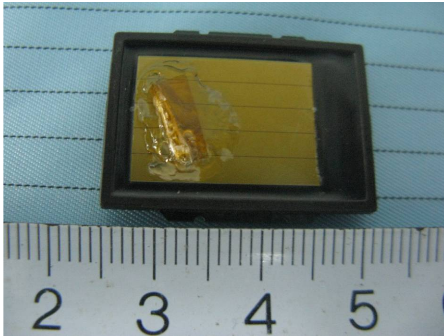
EUT – Fingerprint Board Bottom View
