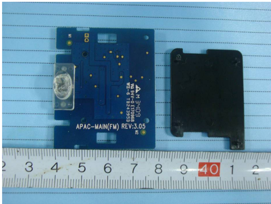
EUT – APAC-Main Board (FM) Bottom Uncovered View
