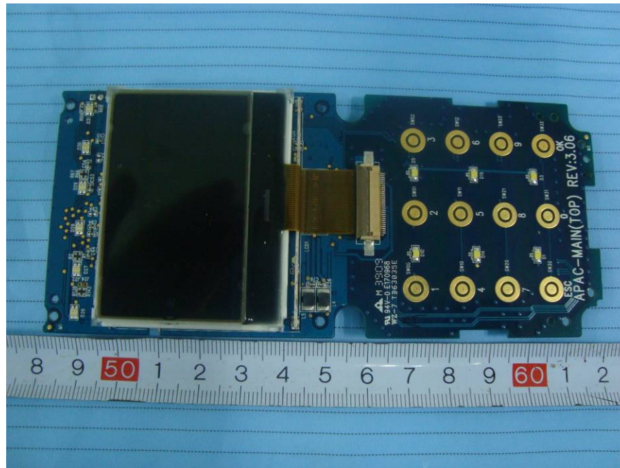
EUT – APAC-Main Board REV3.06 With LCD Top View
