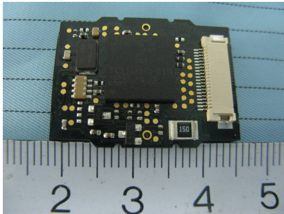
EUT – Fingerprint Board Top View
