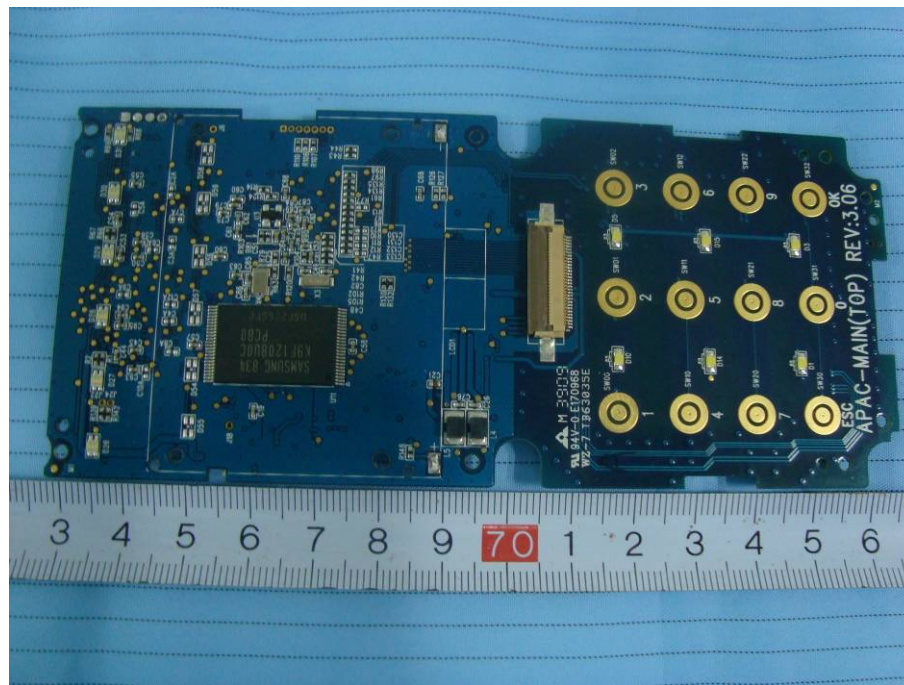
EUT – APAC-Main Board REV3.06 Top View
