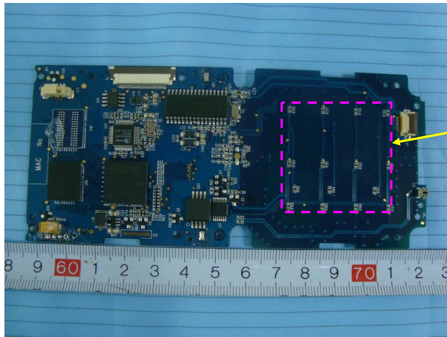
EUT – APAC-Main Board REV3.06 Bottom View
