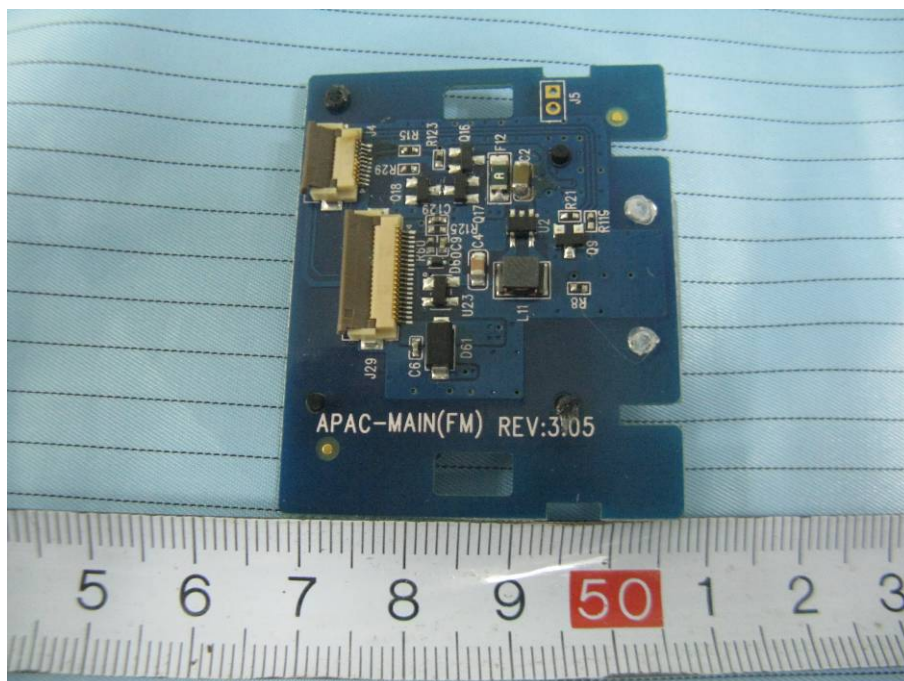
EUT – APAC-Main Board (FM) Top View
