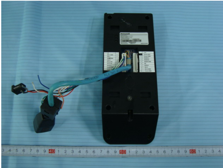
EUT - Rear View (BTFPT)
