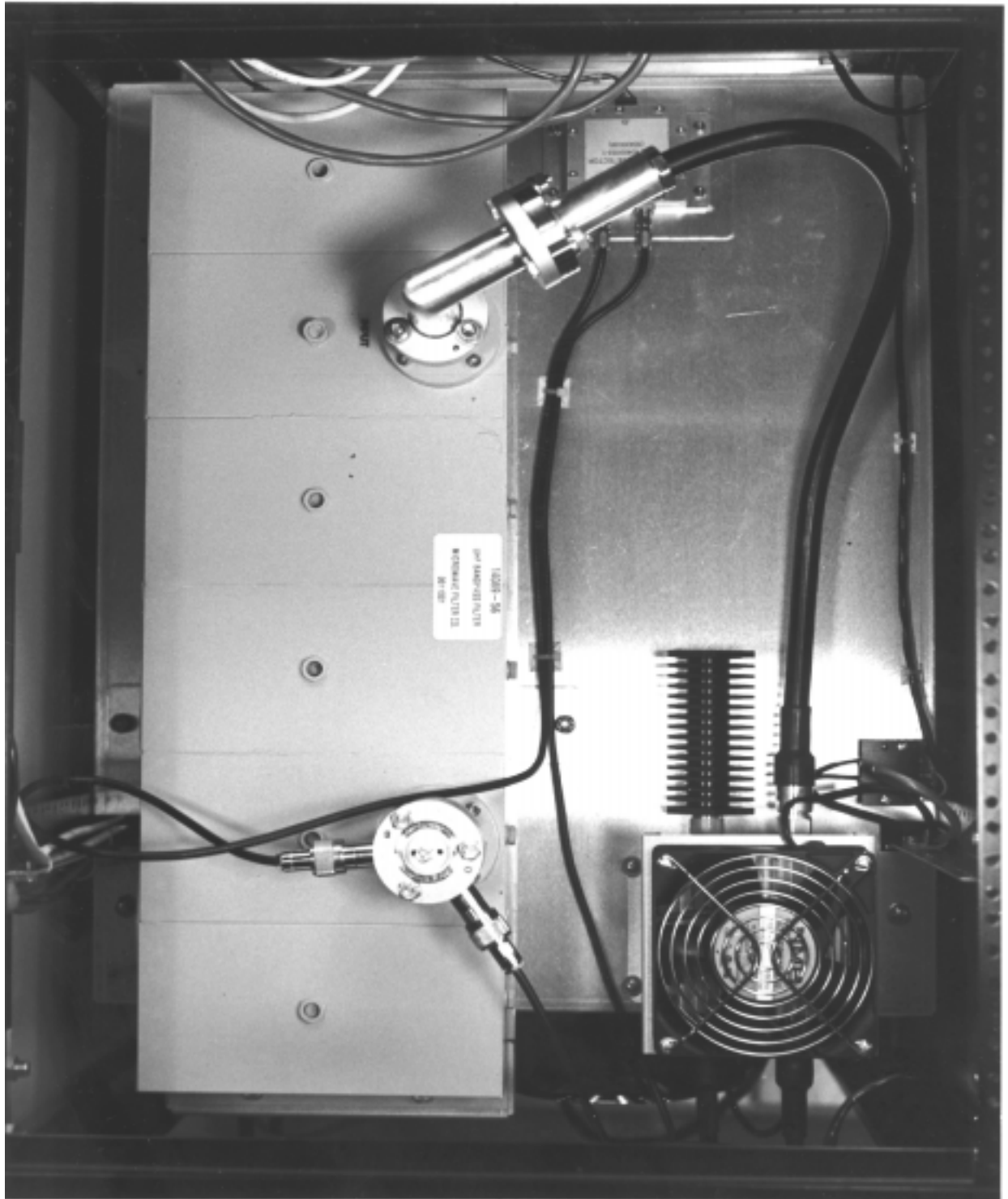
Transmitter Cabinet Top Power Detector and UHF Bandpass Filter
