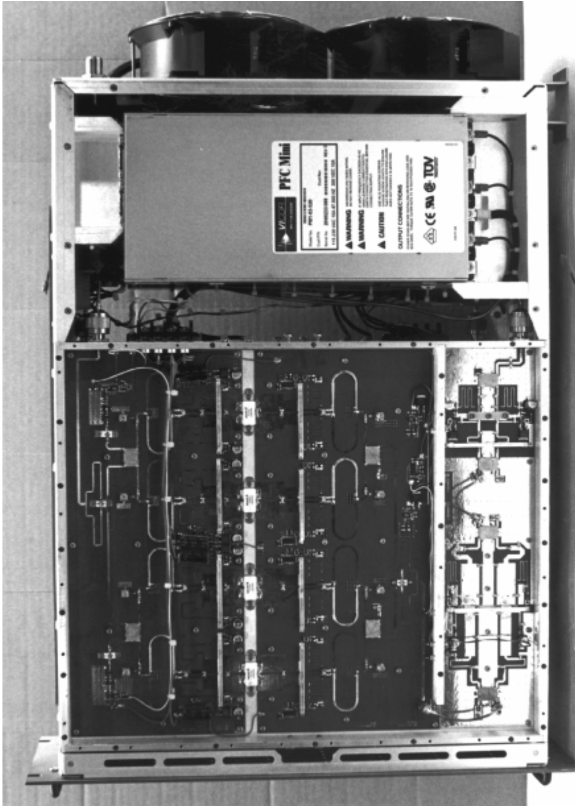
500W UHF Amplifier Drawer Top Side
