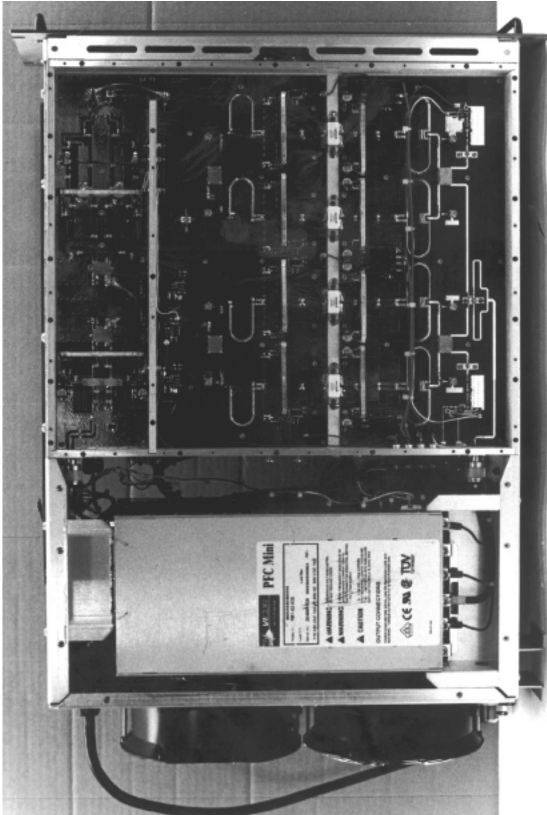
500W UHF Amplifier Drawer Bottom Side
