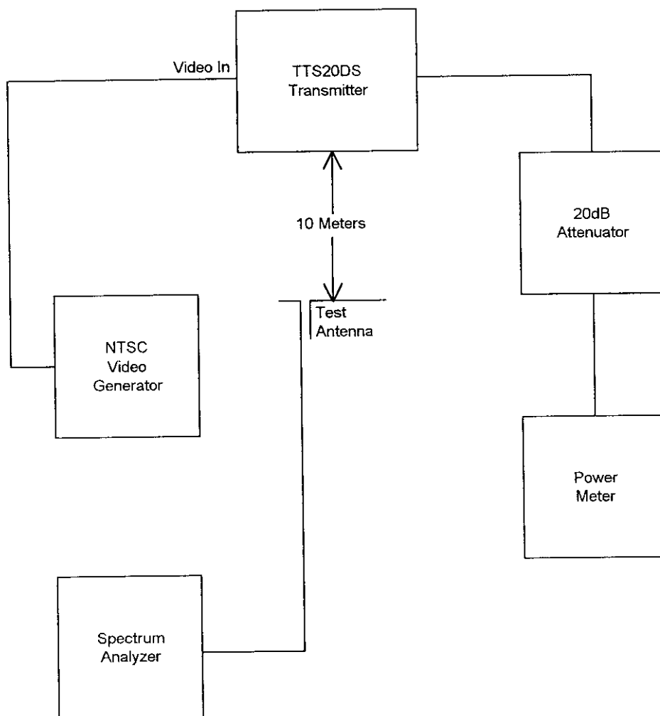
SPURIOUS CABINET RADIATION TEST SETUP Figure 2-11A
