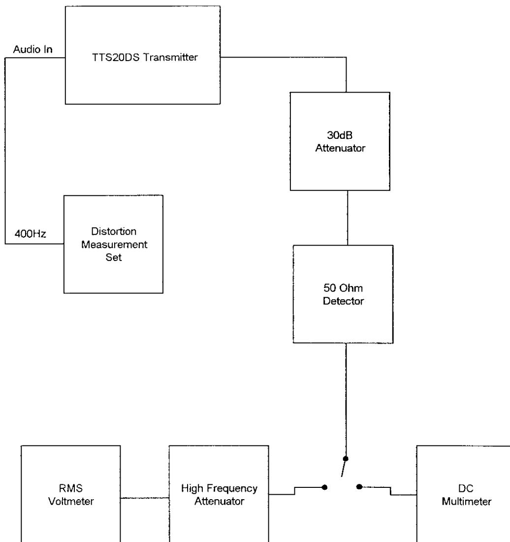
AM NOISE TEST SETUP
