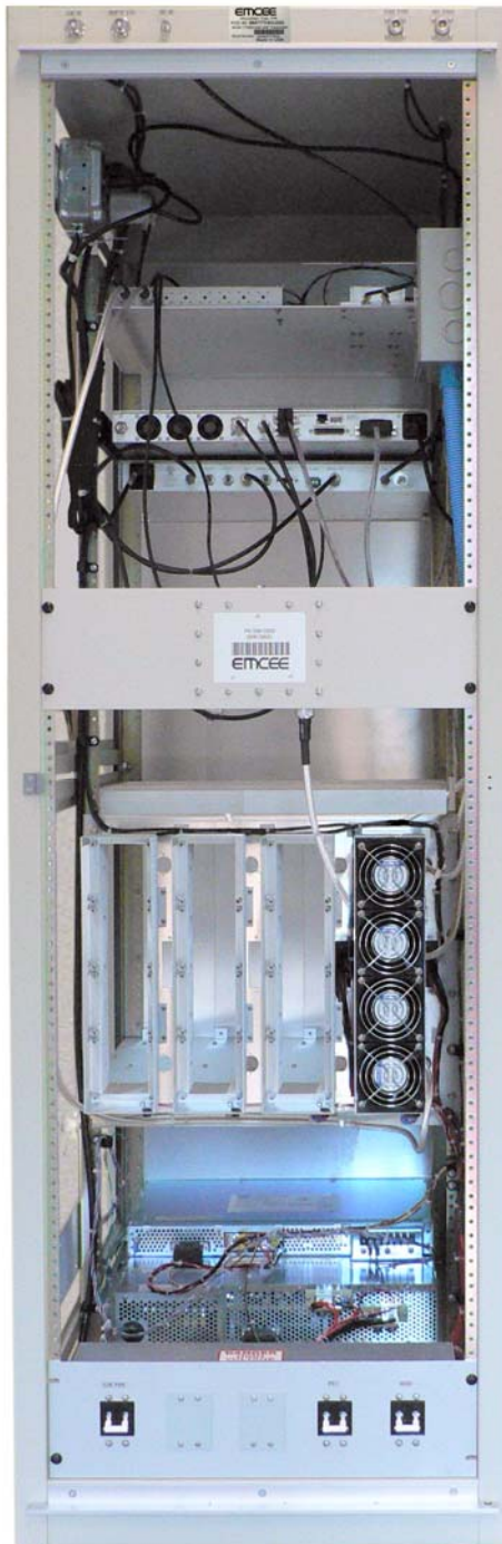
TTHDU-250 Rear View
