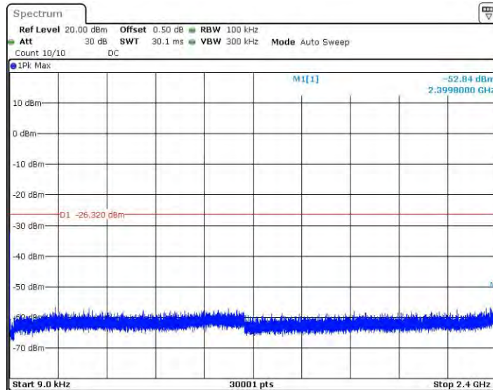
11G_Ant2_2412_0.009~2400
