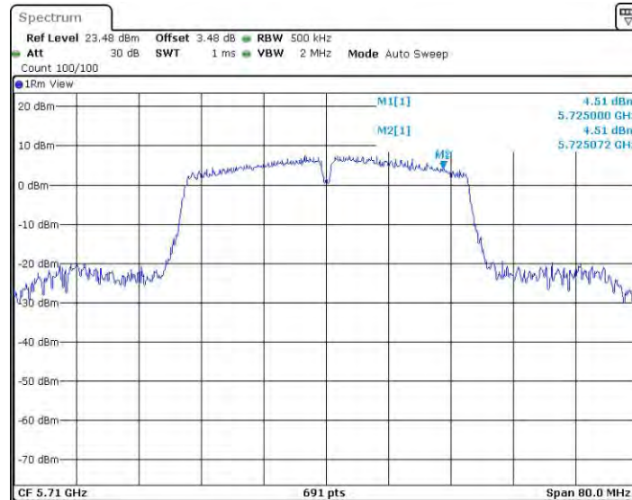
11N40SISO_Ant2_5710_UNII-3
