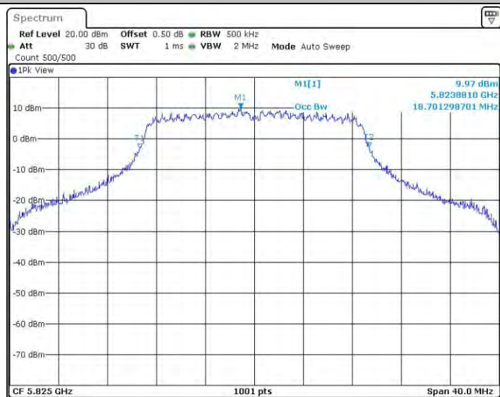
11AC20SISO_Ant2_5825
