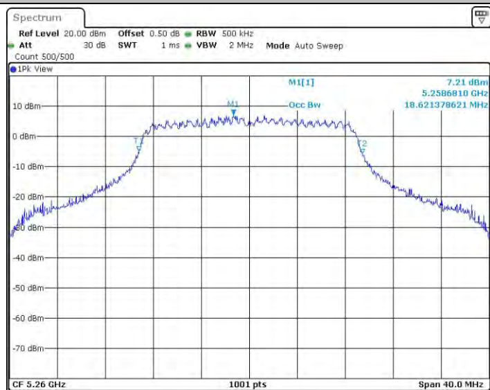
11AC20SISO_Ant2_5260
