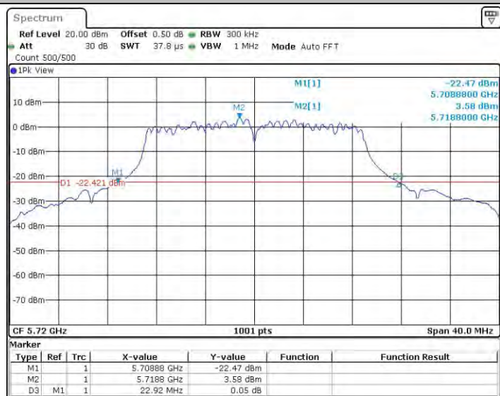
11AC20SISO_Ant1_5720
