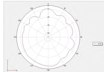
Theta =90 freq=5150MHz
