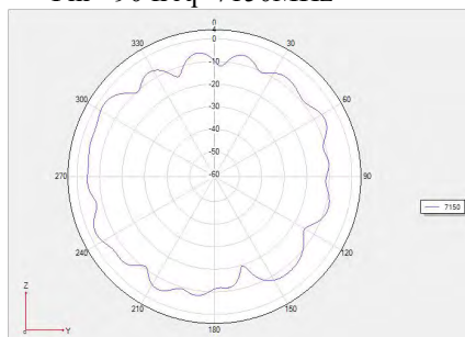
Phi =90 freq=7150MHz
