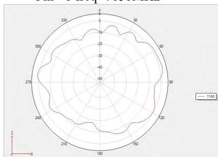
Phi =0 freq=7150MHz
