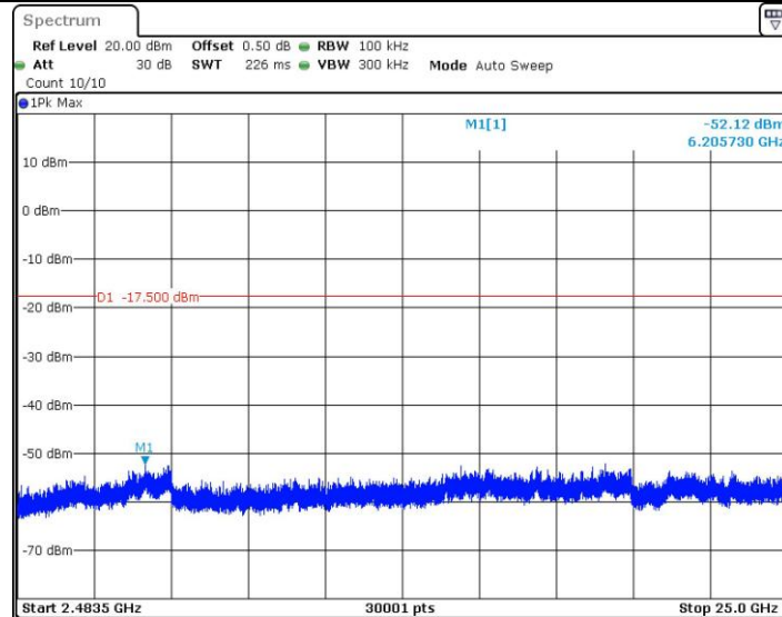
BLE_1M_2402_2483.5~25000
