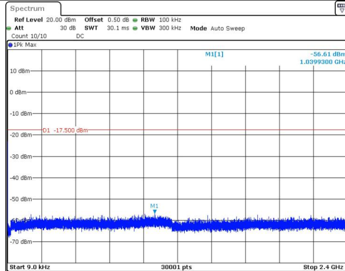
BLE_1M_2402_0.009~2400
