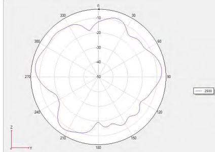
Phi =90 freq=2500MHz
