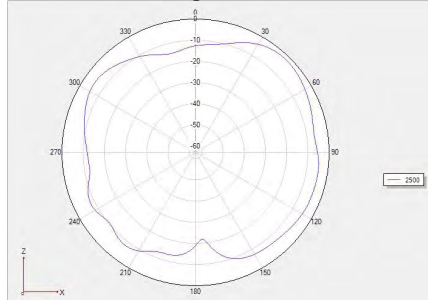
Phi =0 freq=2500MHz
