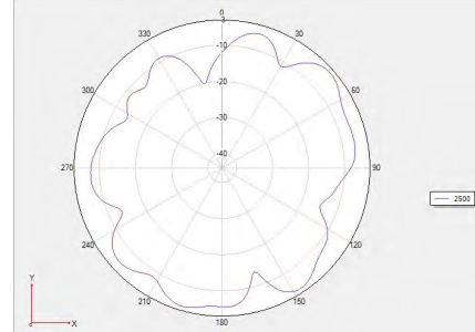
Theta =90 freq=2500MHz
