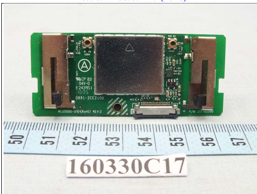
Module: WLU5000-D101(RoHS)
