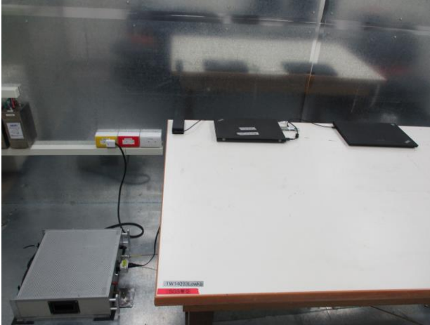
Part_15_407_5G_Conduction_Setup
