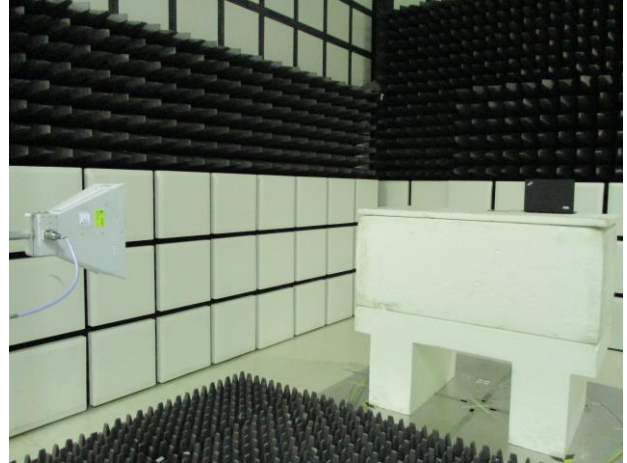
Part_15_407_6E_Radiated_Setup
