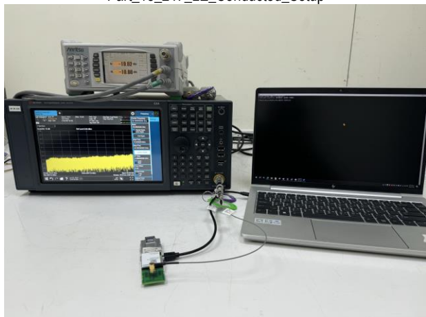
Part_15_247_LE_Conducted_Setup
