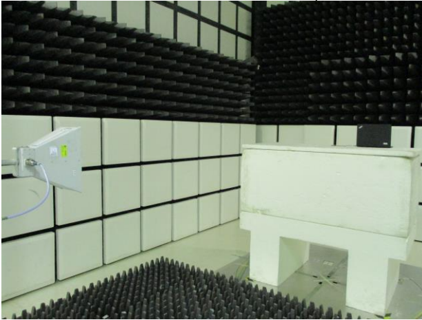
Part_15_247_2.4G_Radiated_Setup
