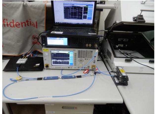
Part_15_407_5G_Normal_DFS_Setup
