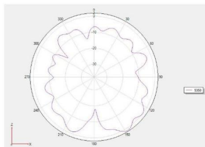
Phi =0 freq=5350MHz
