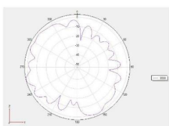
Phi =90 freq=5500MHz
