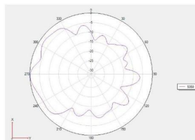
Theta =90 freq=5350MHz
