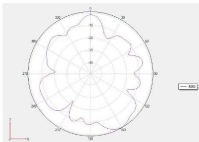
Phi =0 freq=5850MHz
