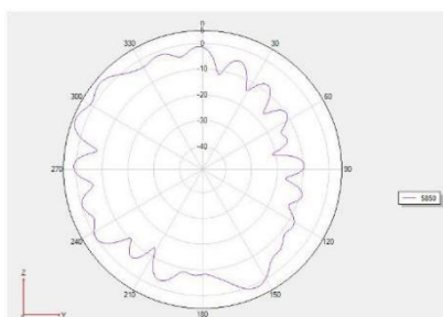
Phi =90 freq=5850MHz
