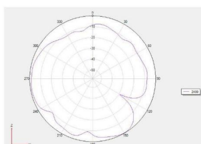
Phi =90 freq=2400MHz
