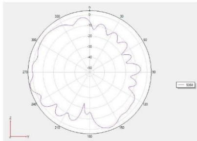
Phi =90 freq=5350MHz
