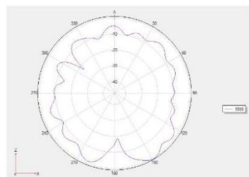
Phi =0 freq=5500MHz
