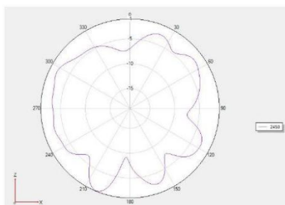
Phi =0 freq=2450MHz
