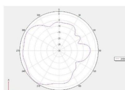
Theta =90 freq=2450MHz
