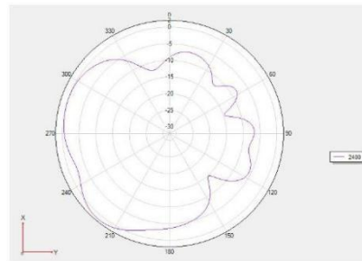
Theta =90 freq=2400MHz
