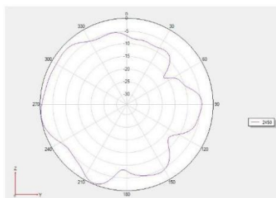
Phi =90 freq=2450MHz
