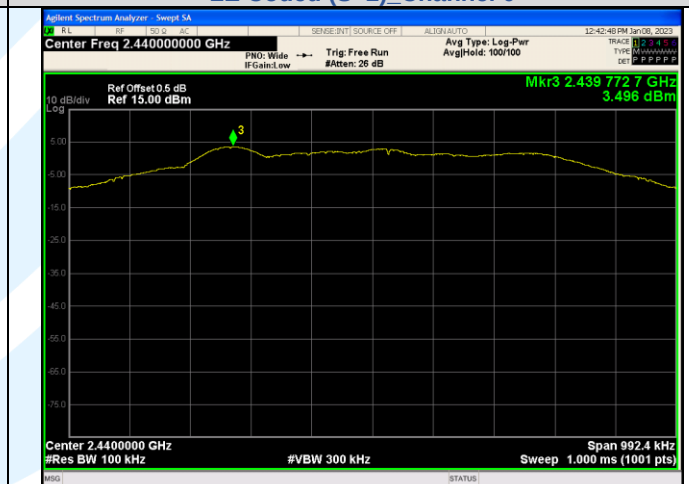
In-Band Reference Level LE Coded (S=2)_Channel 19
