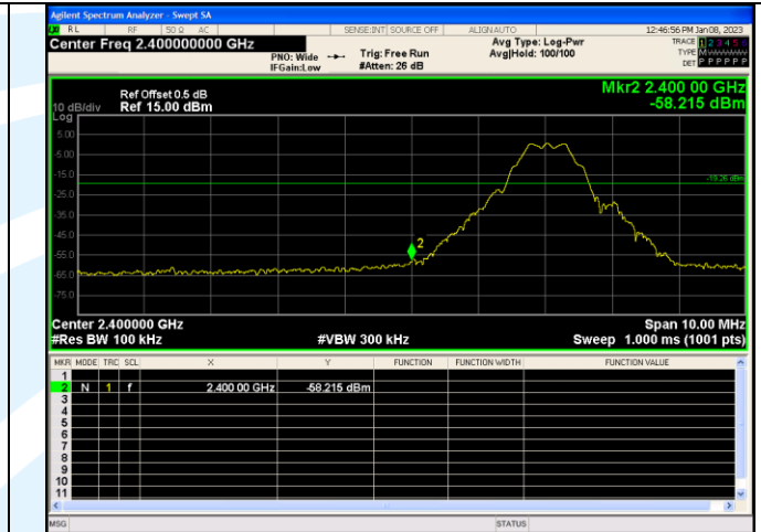
Out Of Band Emission LE Coded (S=8)_Channel 0
