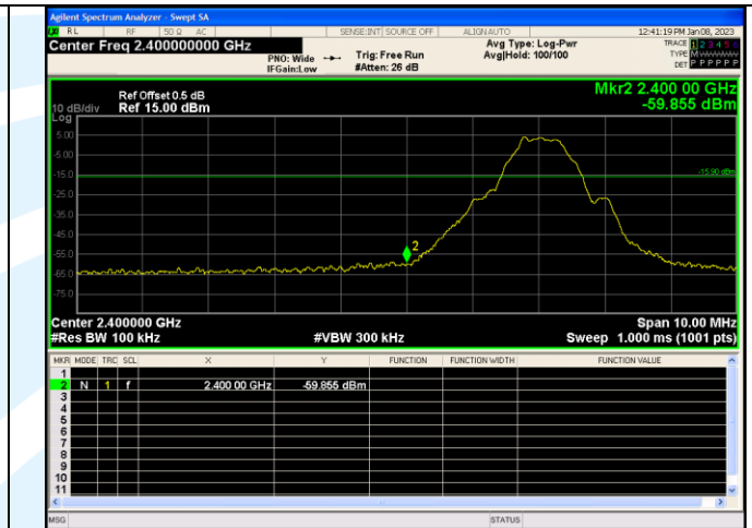
Out Of Band Emission LE Coded (S=2)_Channel 0
