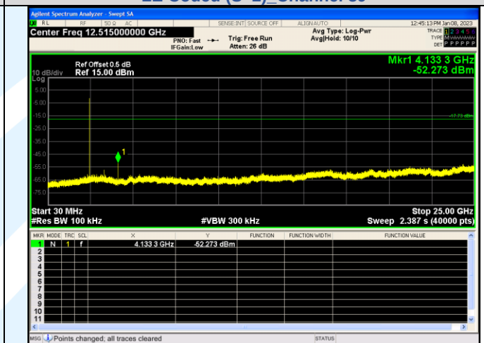
Spurious Emission LE Coded (S=2) Channel 39
