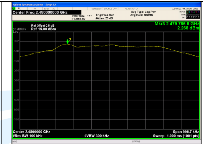
In-Band Reference Level LE Coded (S=2) Channel 39
