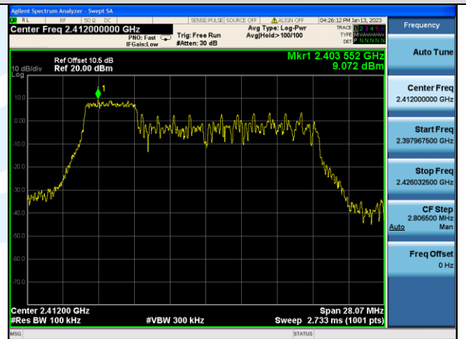
In-Band Reference Level IEEE 802.11ax_Channel 1_20MHz_Antenna 2_RU&Index 52RU37
