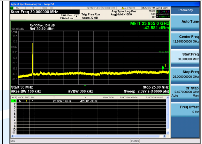
Spurious Emission IEEE 802.11ax_Channel 1_20MHz_Antenna 2_RU&Index 52RU37
