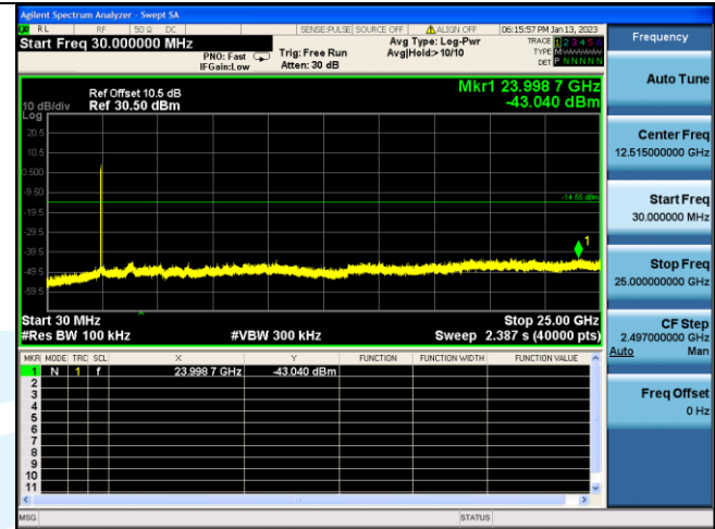
Spurious Emission IEEE 802.11ax_Channel 11_20MHz_Antenna 2_RU&Index 106RU54
