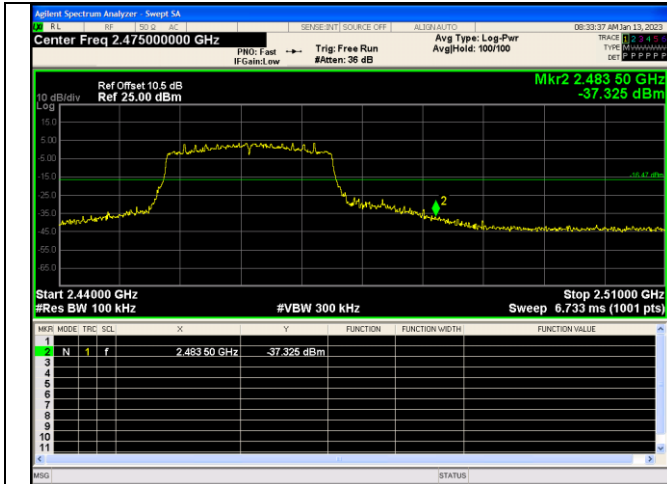
Out Of Band Emission IEEE 802.11ax_Channel 11_20MHz_Antenna 2_RU&Index SU
