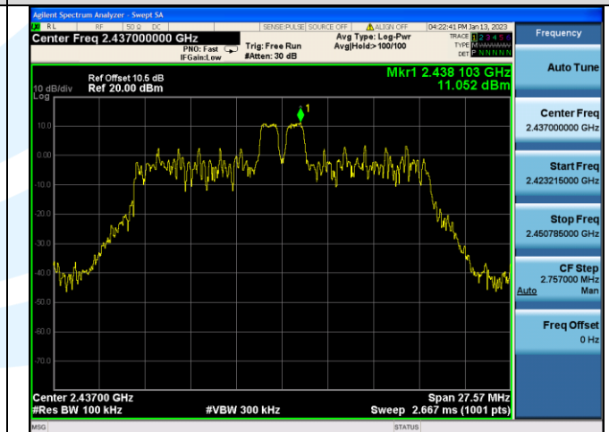
In-Band Reference Level IEEE 802.11ax_Channel 6_20MHz_Antenna 2_RU&Index 26RU4
