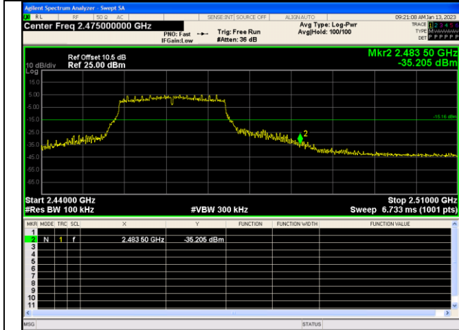
Out Of Band Emission IEEE 802.11n Channel 11 20MHz Antenna 2
