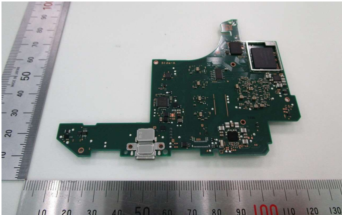
Wireless module PCB (Back):
