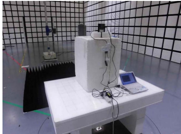
above 1 GHz
