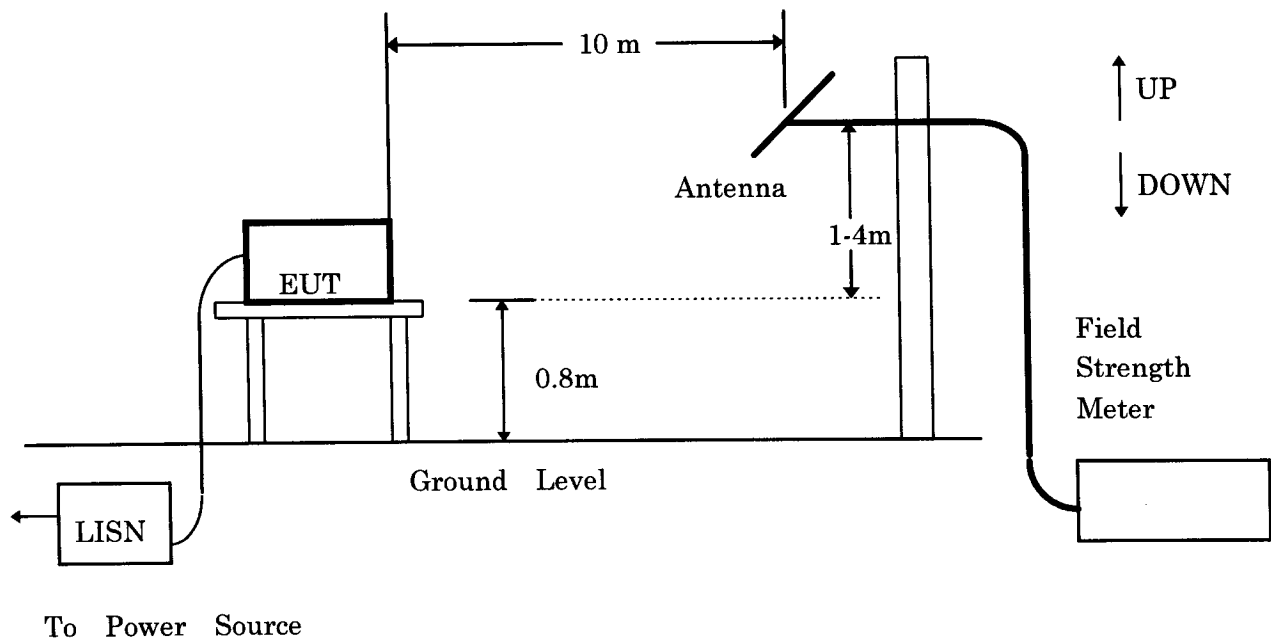
TSET SET-UP SKETCH
