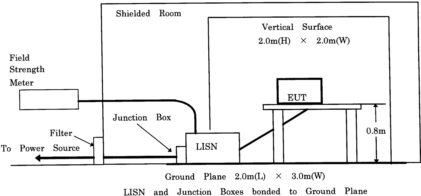
TEST SET-UP SKETCH
