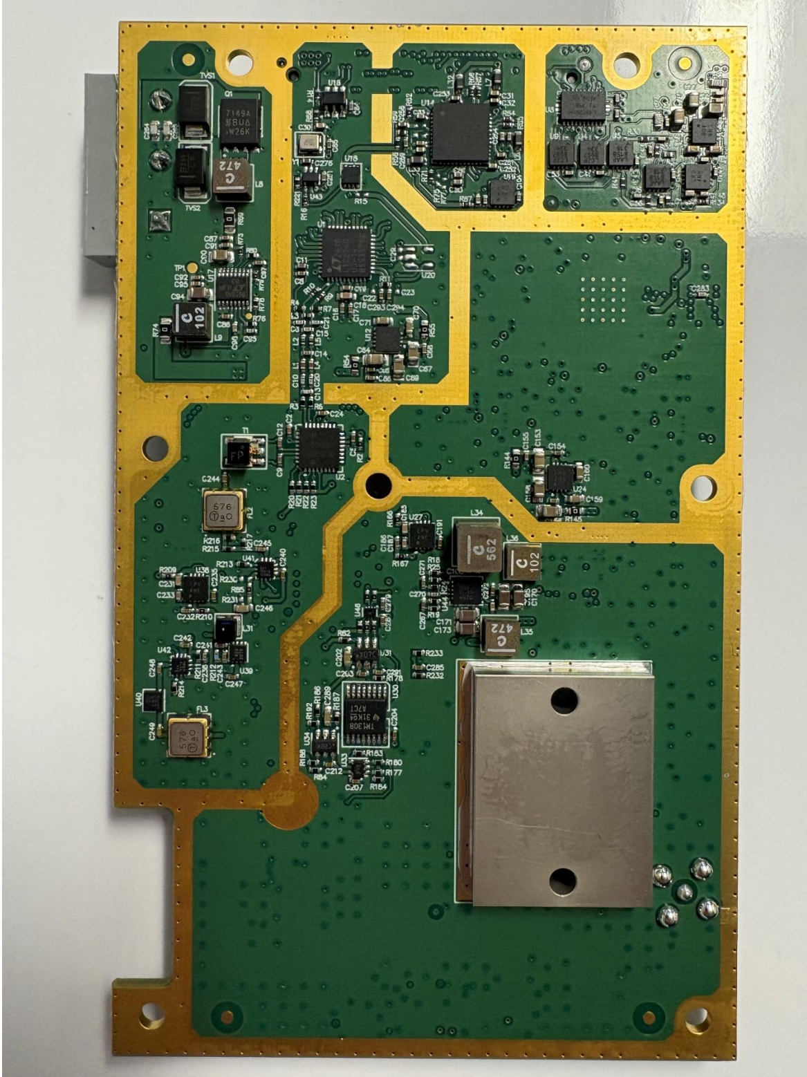
Figure 1 - RF Board - Bottom Side
