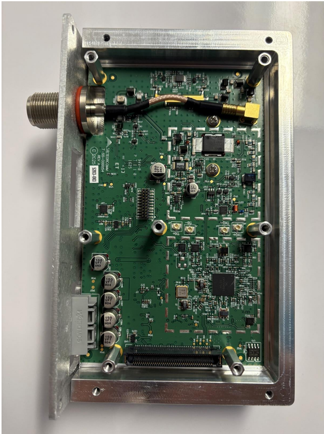
Figure 6 - Assembly with main board removed
