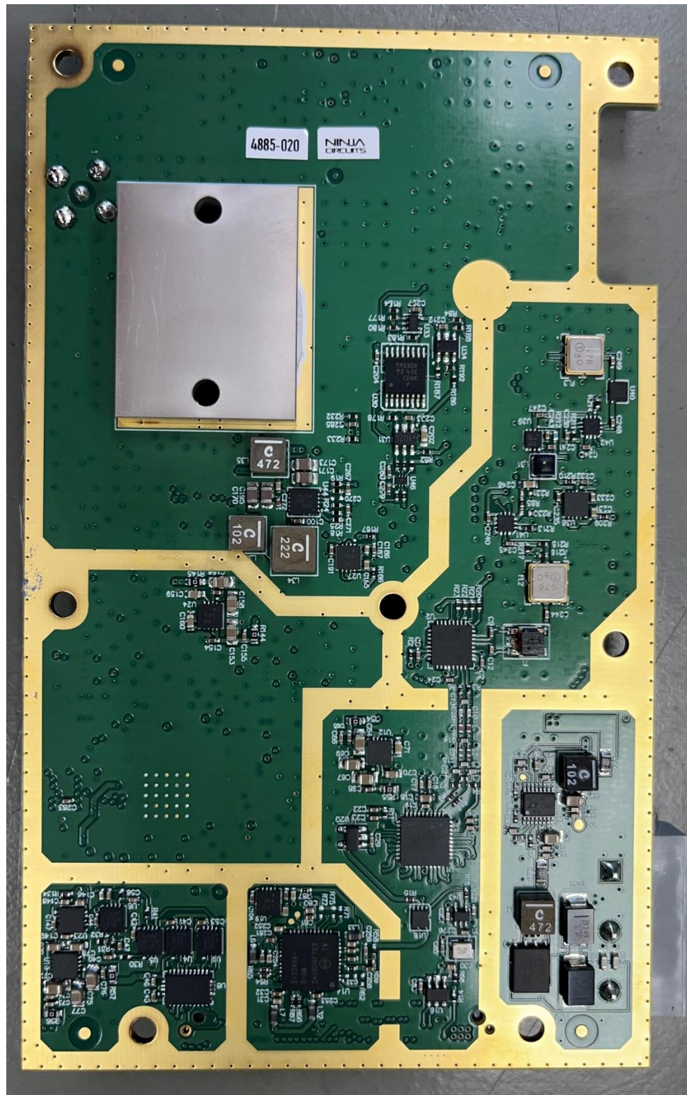
Figure 2 - RF Board – Top Side
