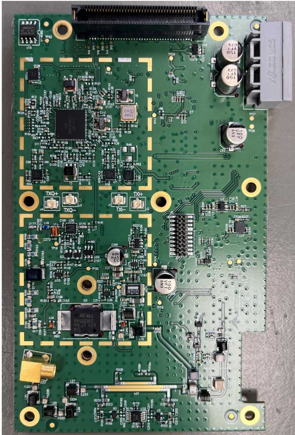
Figure 1 - RF Board - Bottom Side
