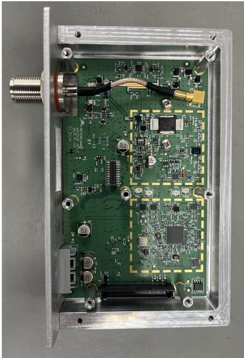
Figure 6 - Assembly with main board removed
