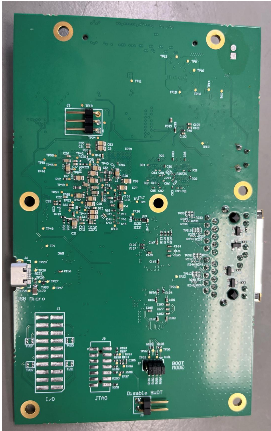
Figure 4 - Main Board – Top Side
