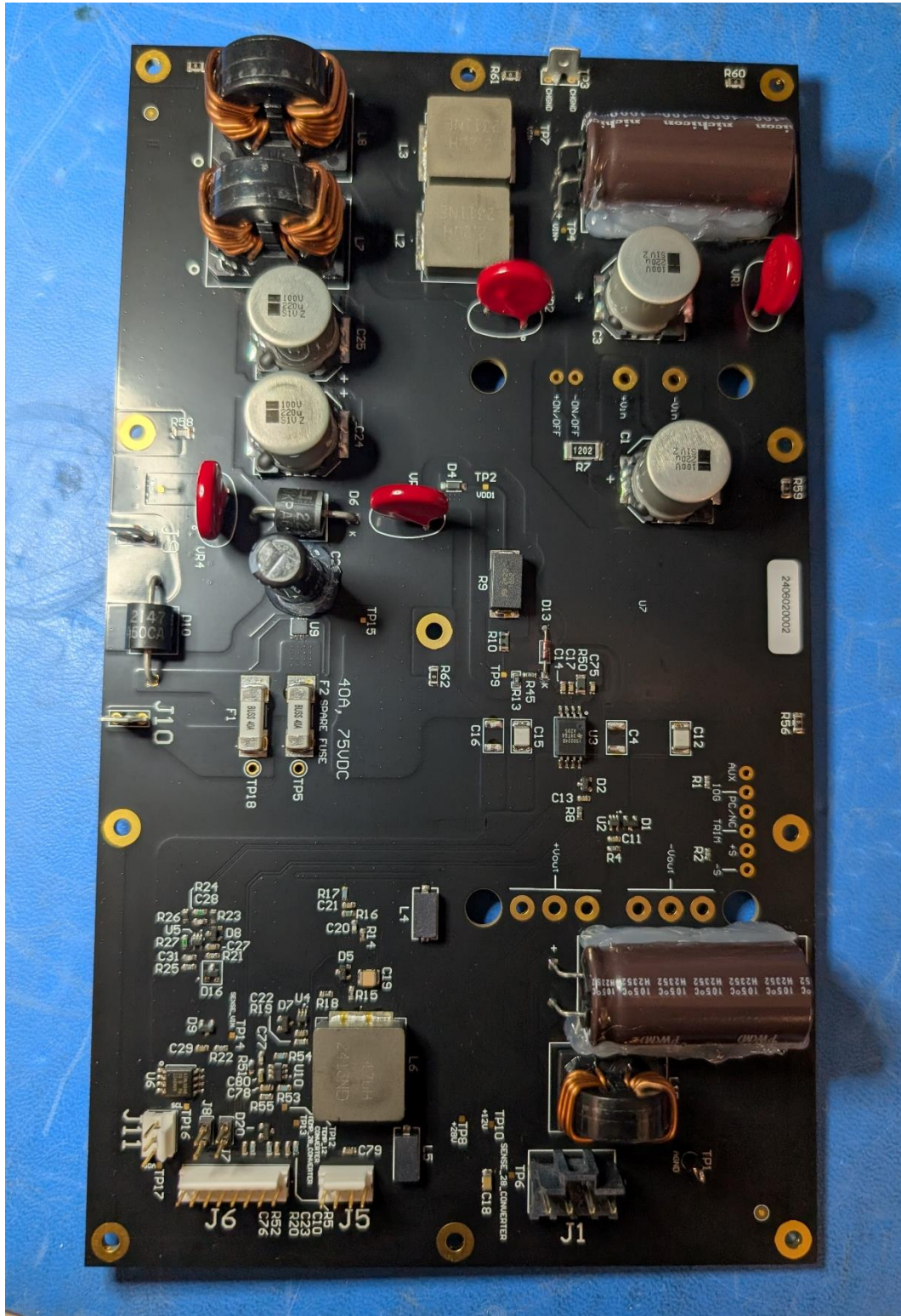
Figure 11– Power Supply Board - Top Side
