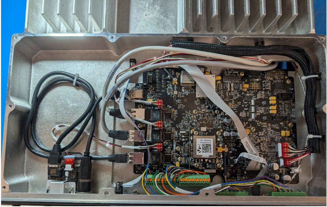
Figure 15 - Assembly top view
