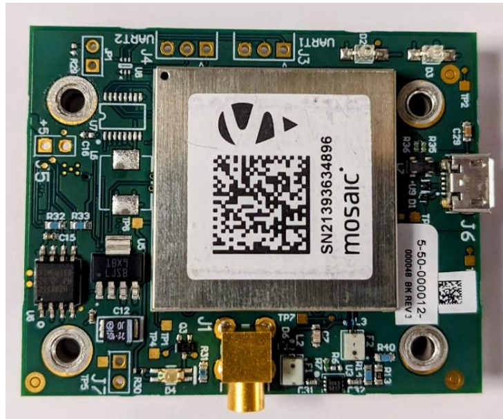
Figure 13- GNSS Board - Top Side
