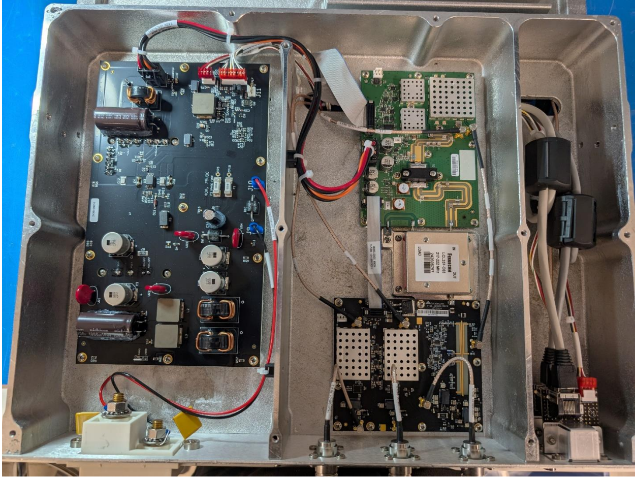
Figure 16 - Assembly Bottom view
