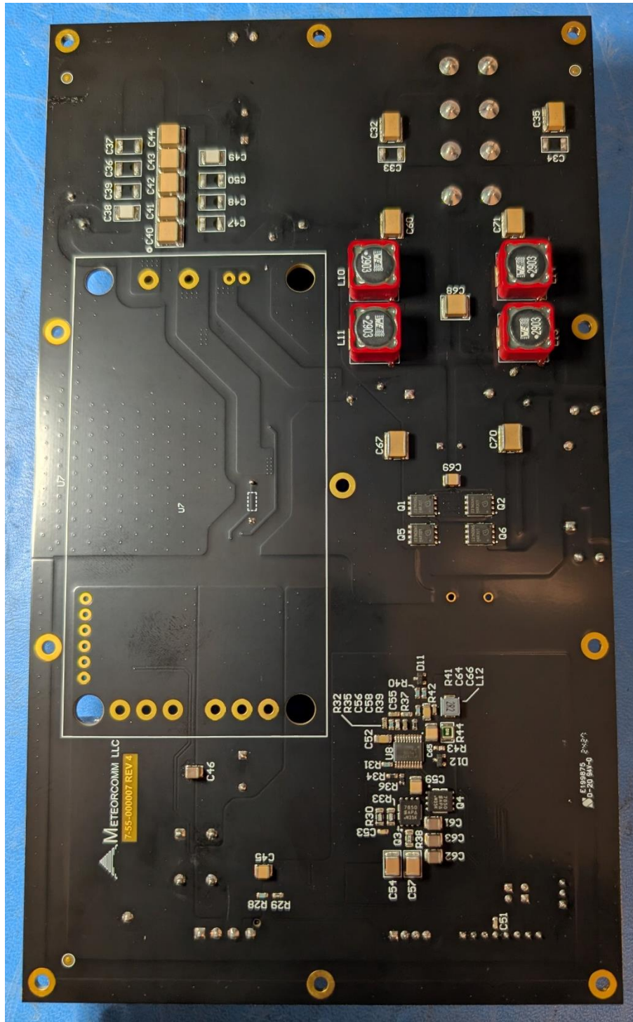
Figure 12 – Power Supply Board - Top Side
