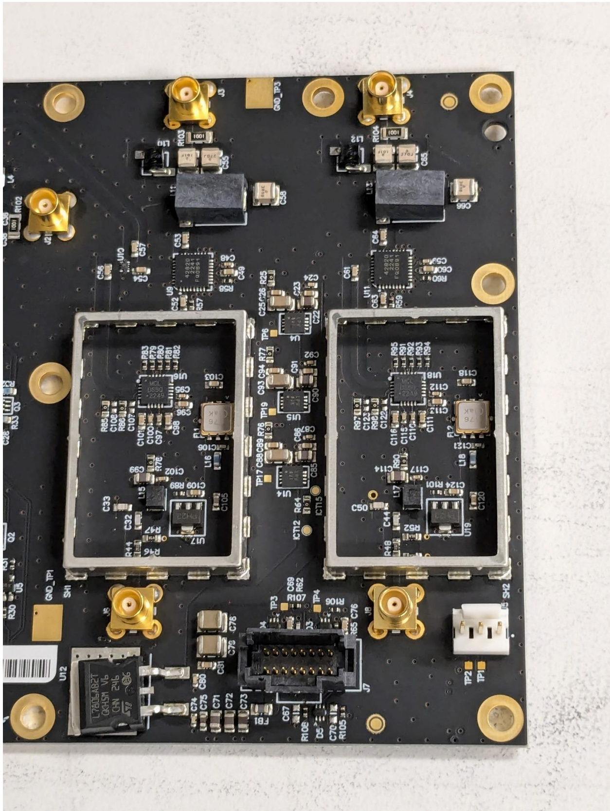
Figure 9 – Front-End Board Top Side, No Cans
