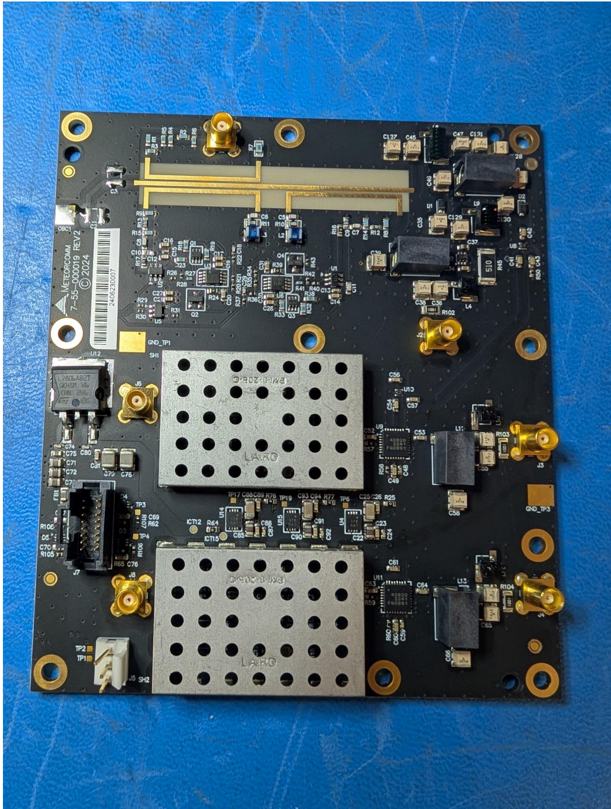
Figure 8 – Front-End Board Top Side
