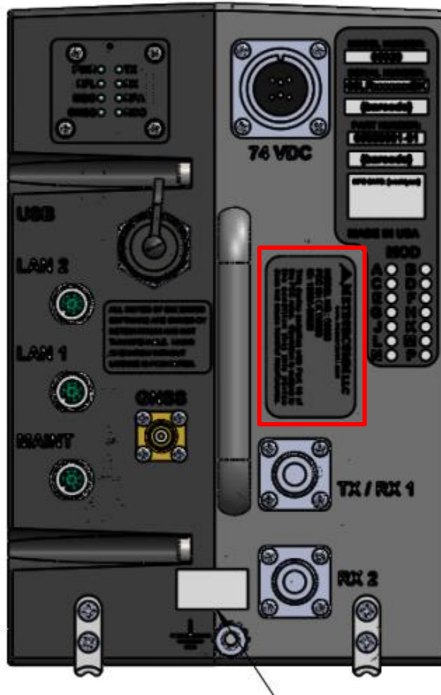
Figure 2 - Model - Location of the FCC/IC label on the front of the radio
