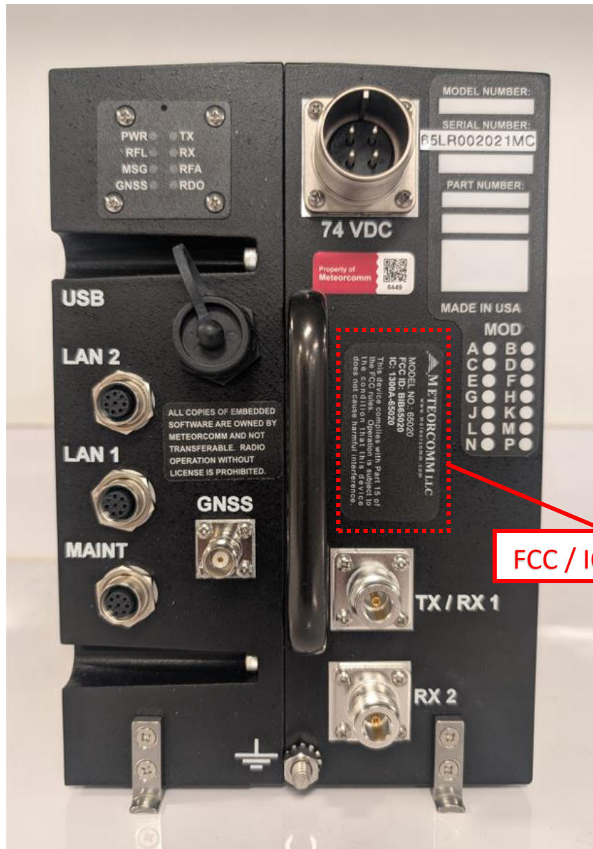
Figure 4 - ITCRNG Loco Radio Label placement - photo - front view
