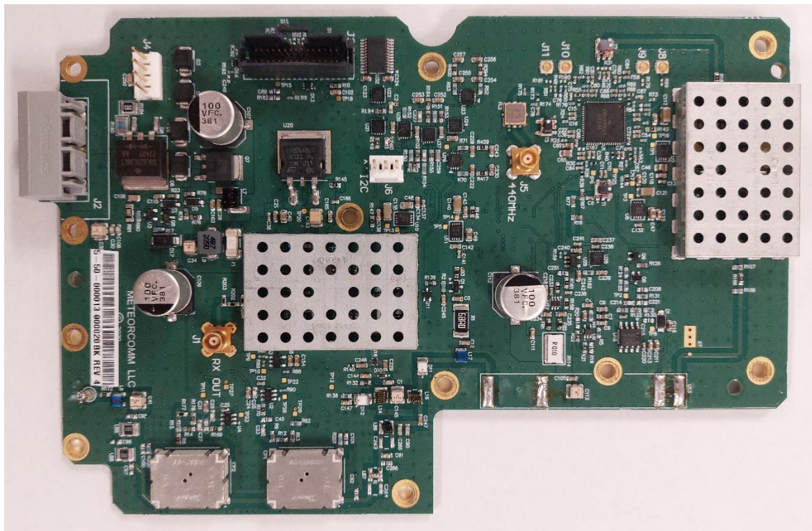
Figure 4 - RF Board - Top Side - Shields on
