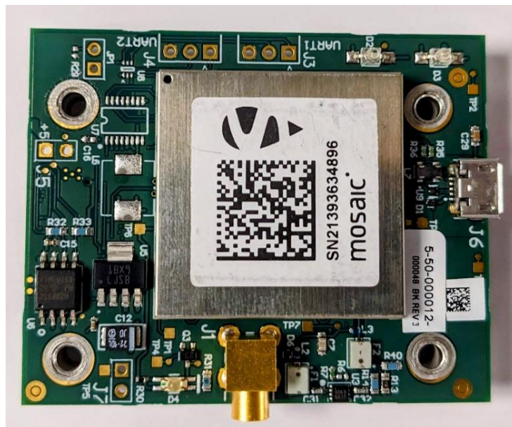
Figure 6- GNSS Board - Top Side
