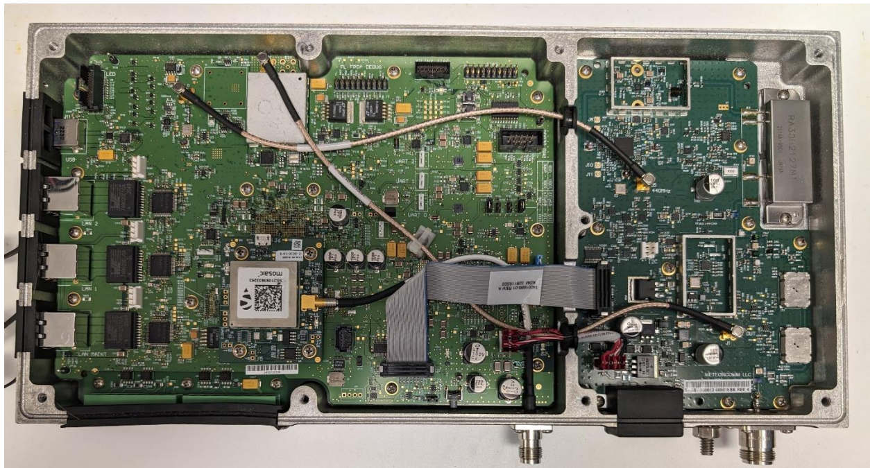
Figure 8 - Assembly top view
