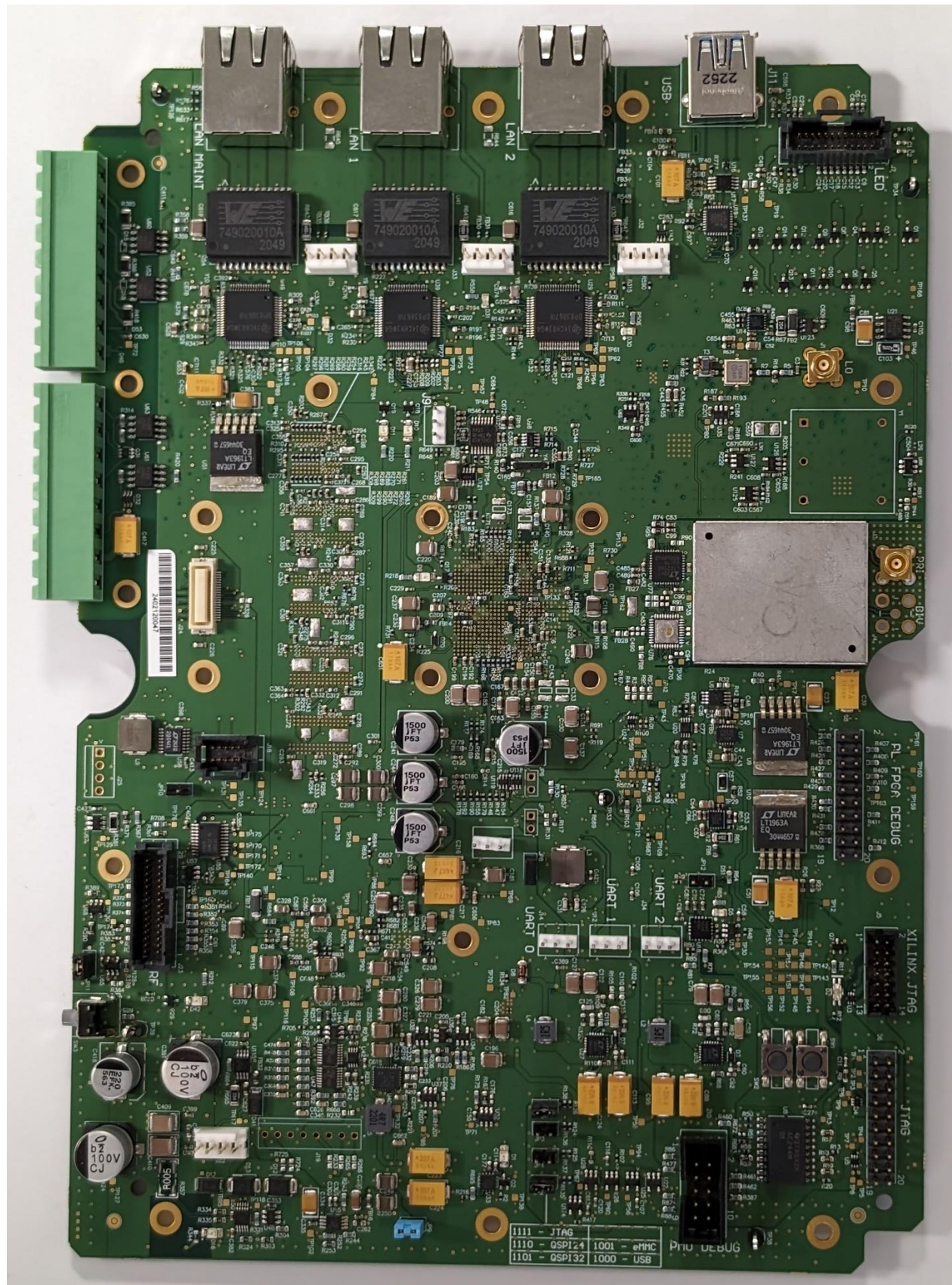
Figure 1 - Main Board - Top Side
