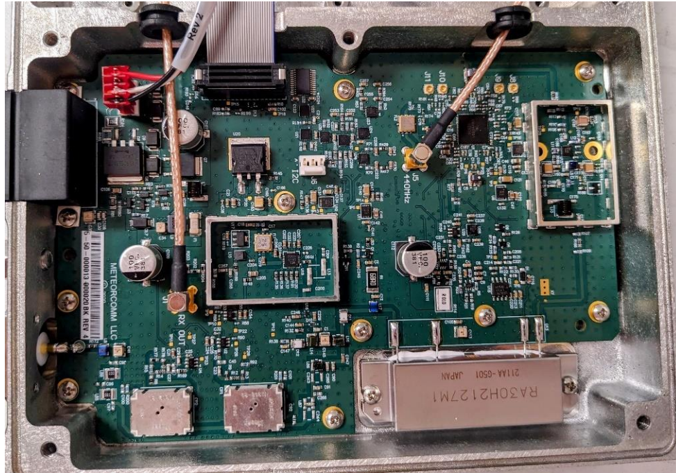
Figure 3 - RF Board - Top Side, no shields
