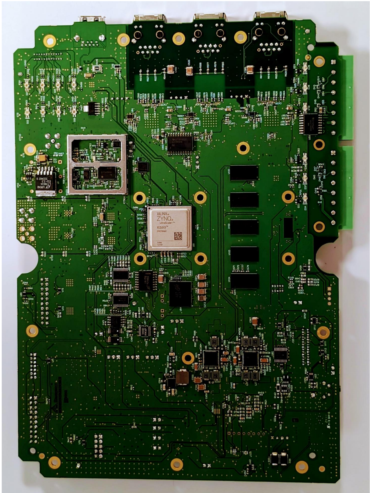
Figure 2 - Main Board – Bottom Side
