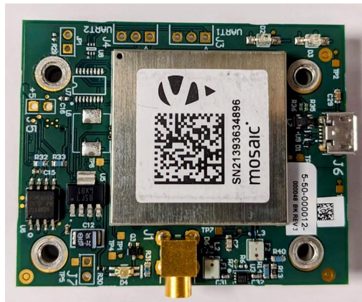
Figure 6- GNSS Board - Top Side
