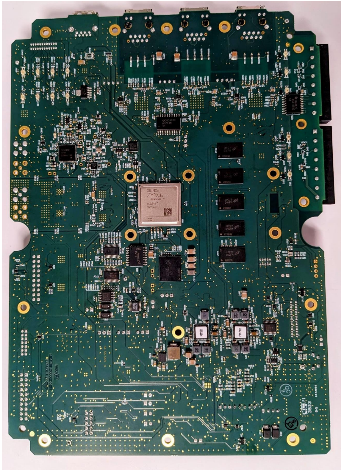
Figure 2 - Main Board – Bottom Side
