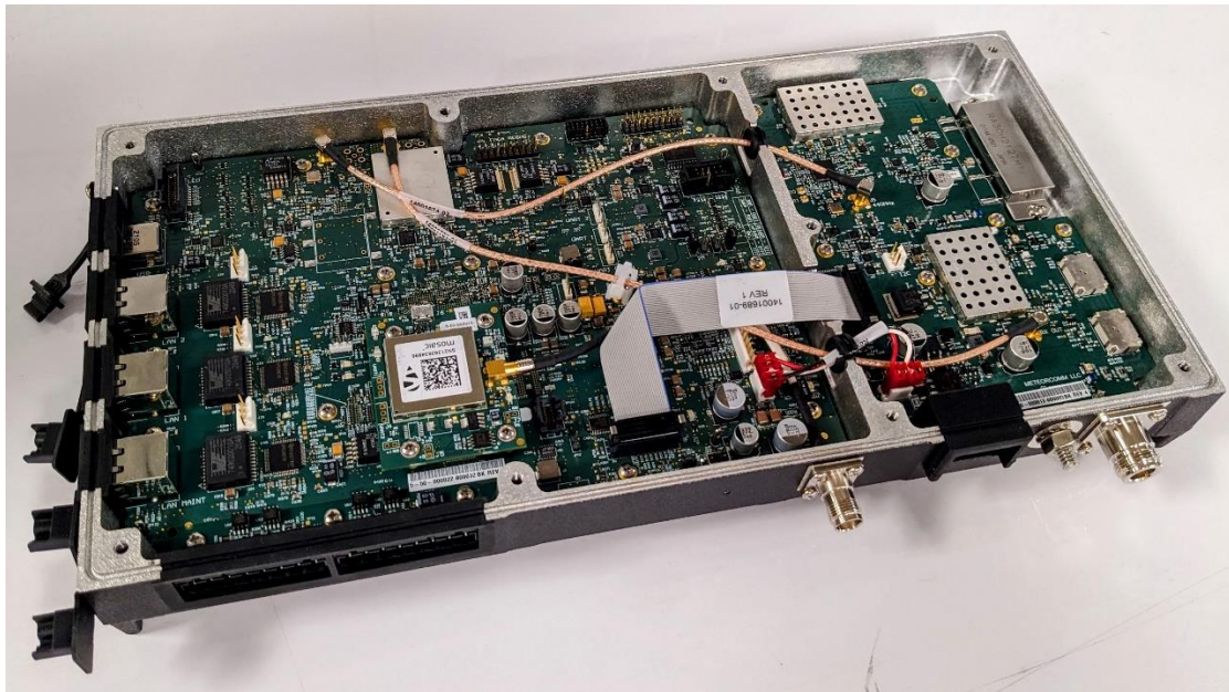
Figure 9 - Assembly, perspective
