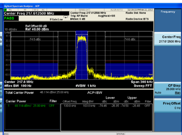
Figure 8C4. fo ± 150 kHz, 100kHz IBW
