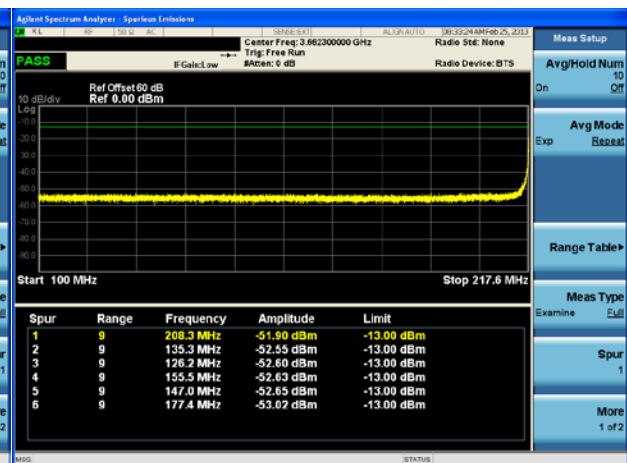
Figure 8C2. 100 to 217.6 MHz, 10 kHz BW
